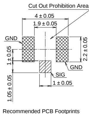
Recommended PCB Footprints
