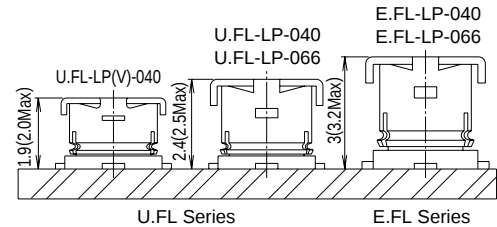
Mated Height Comparison (With Hirose Product)
