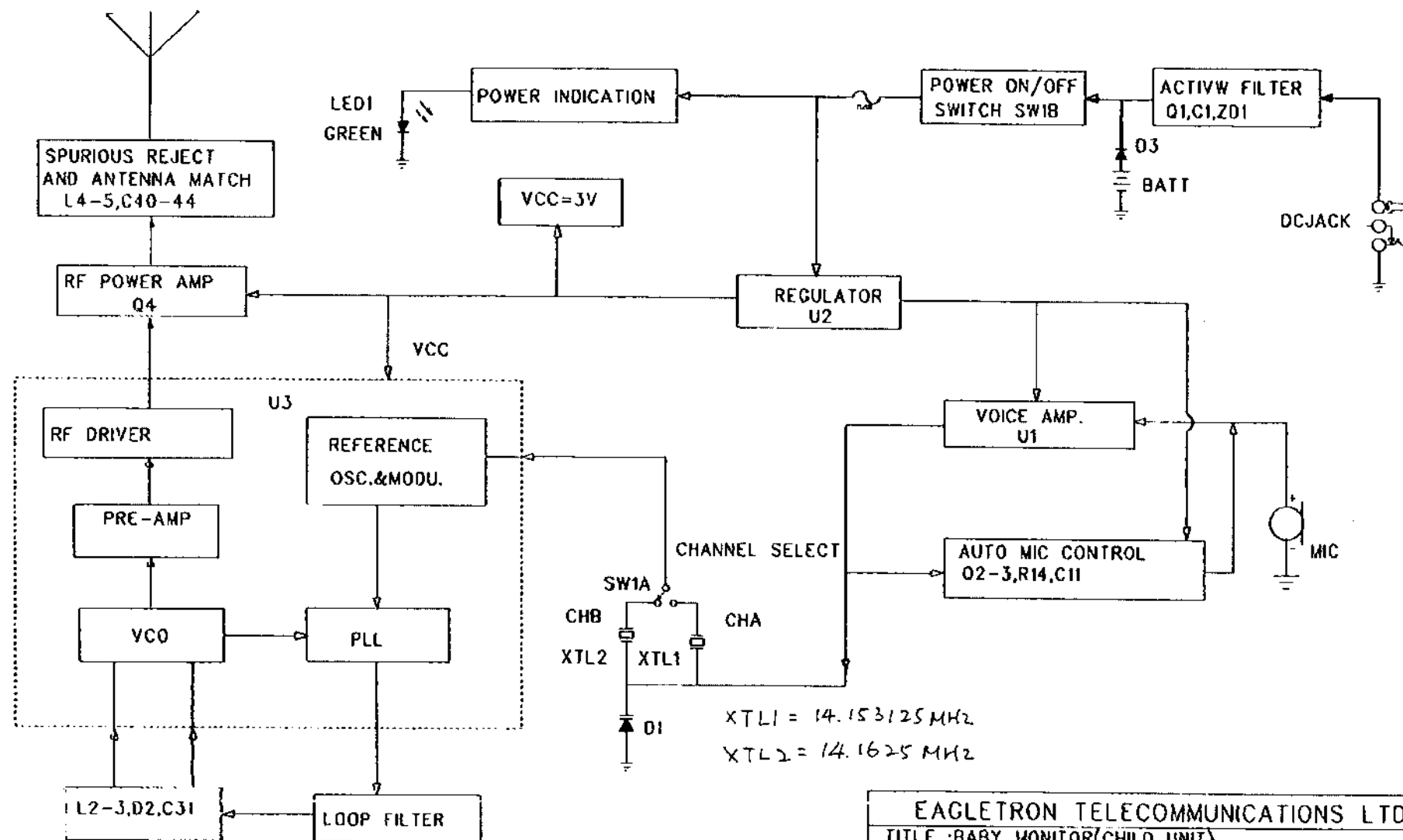
TFY-8814-USA TRANSMITTER
