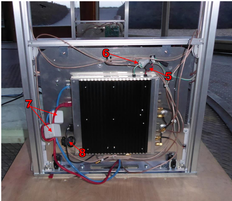
Evolve E10 2.0 ANT RF w/RFID upgrade kit - Master
