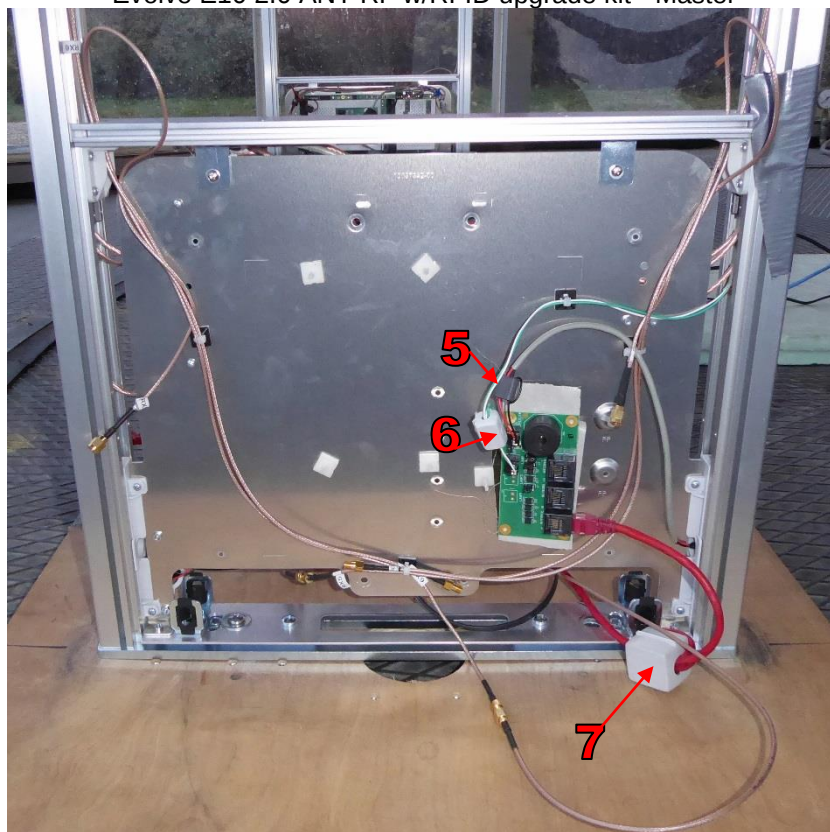
Evolve E10 2.0 ANT RF w/RFID upgrade kit - Master
