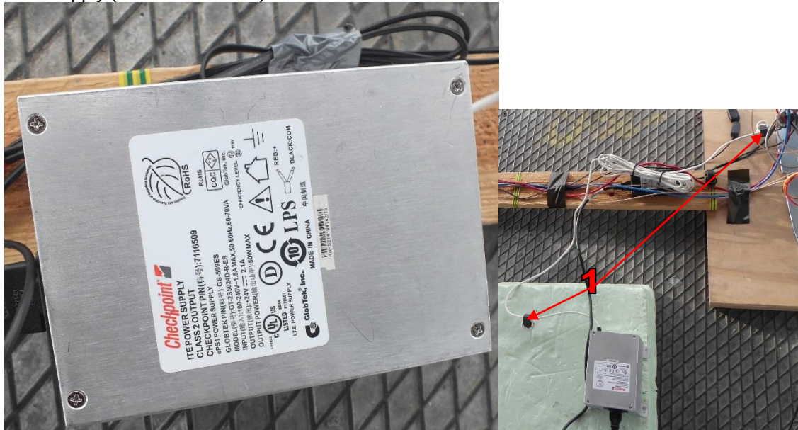
EOS power supply (Evolve electronic):
