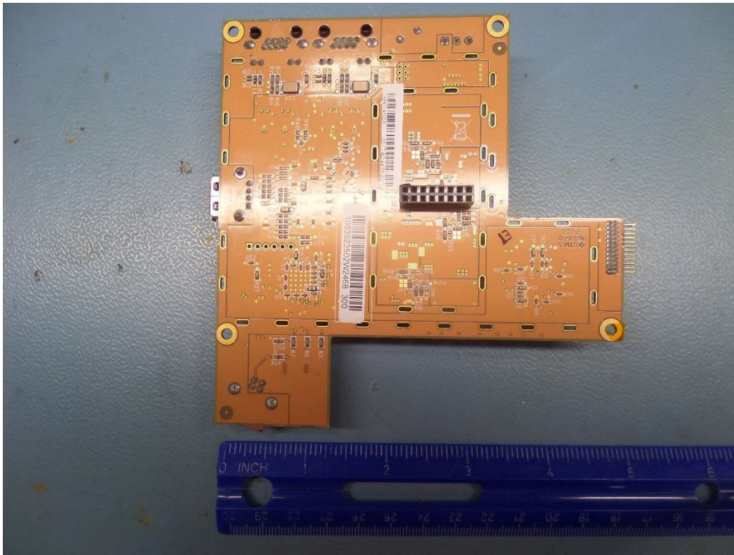
Figure 11: NP10 PAB w/HUB HUB board bottom side
