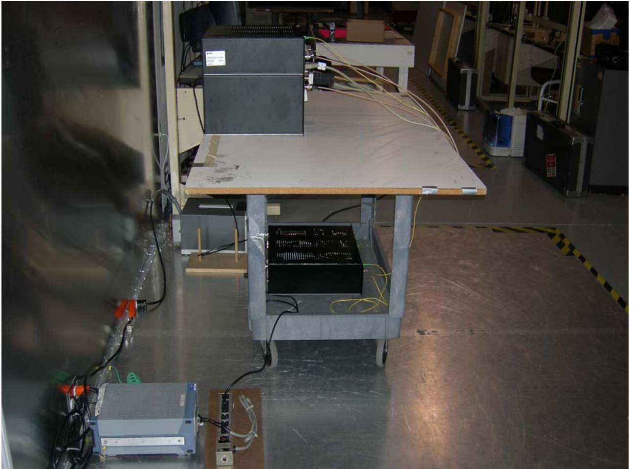
Figure 6: Conducted Emissions
