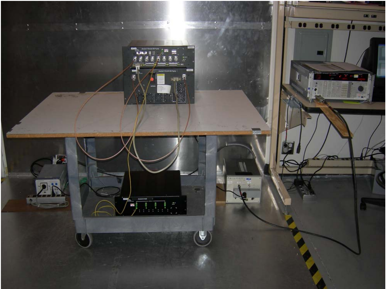
Figure 5: Conducted Emissions
