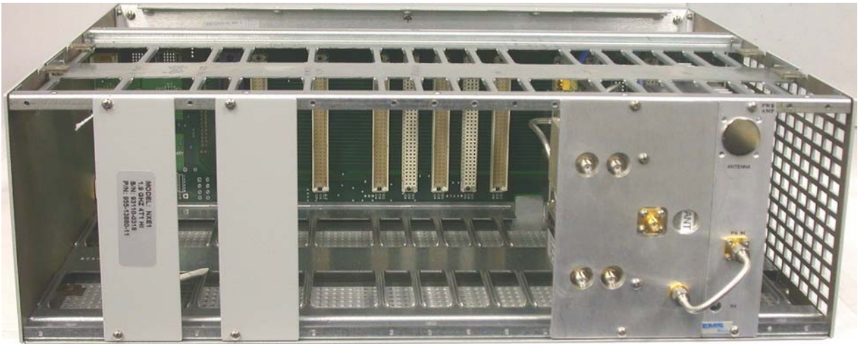
Figure 4: Empty Shell – Rear View 2
