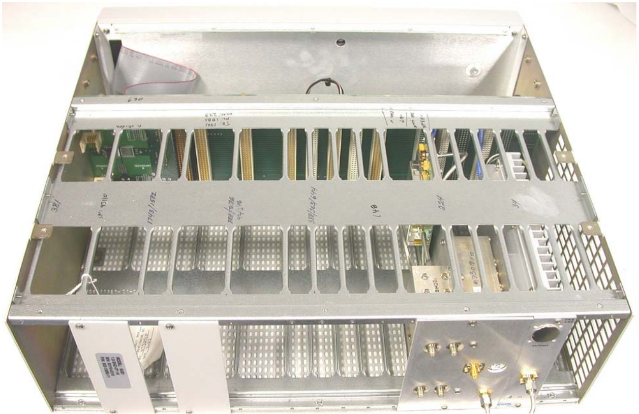
Figure 3: Empty Shell – Rear View
