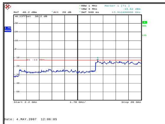
Figure 63: Spurious Emissions - Downlink GSM Mid Channel – 2.2 to 20GHz
