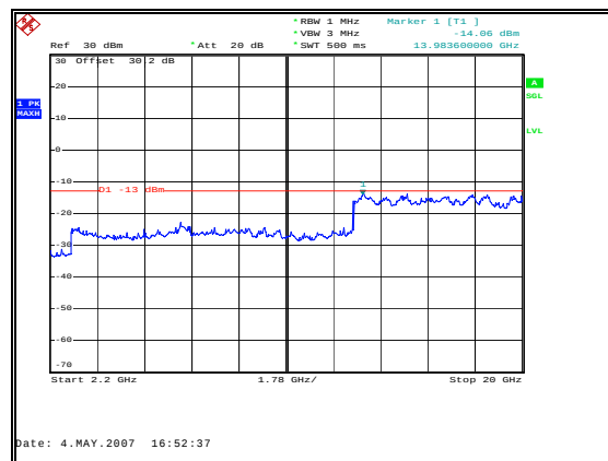
Figure 39: Spurious Emissions - Uplink GSM Mid Channel – 2.2 to 20GHz
