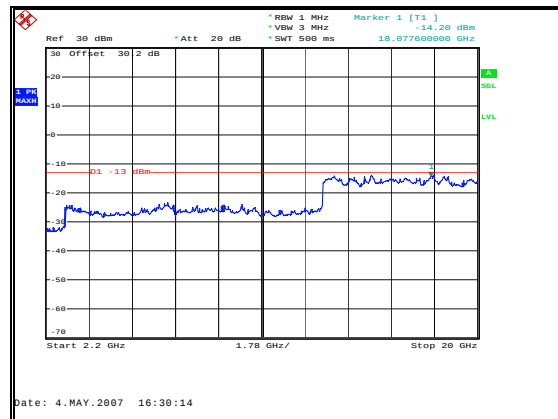
Figure 37: Spurious Emissions - Uplink GSM Low Channel – Inter-modulation – 2.2 to 20GHz
