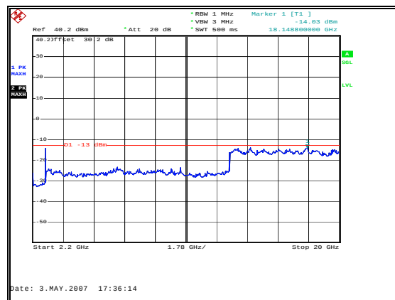
Figure 47: Spurious Emissions - Downlink CDMA Mid Channel – 2.2 to 20GHz
