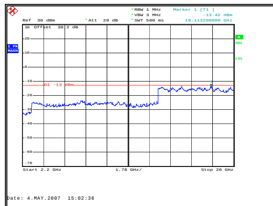
Figure 23: Spurious Emissions - Uplink CDMA Mid Channel – 2.2 to 20GHz
