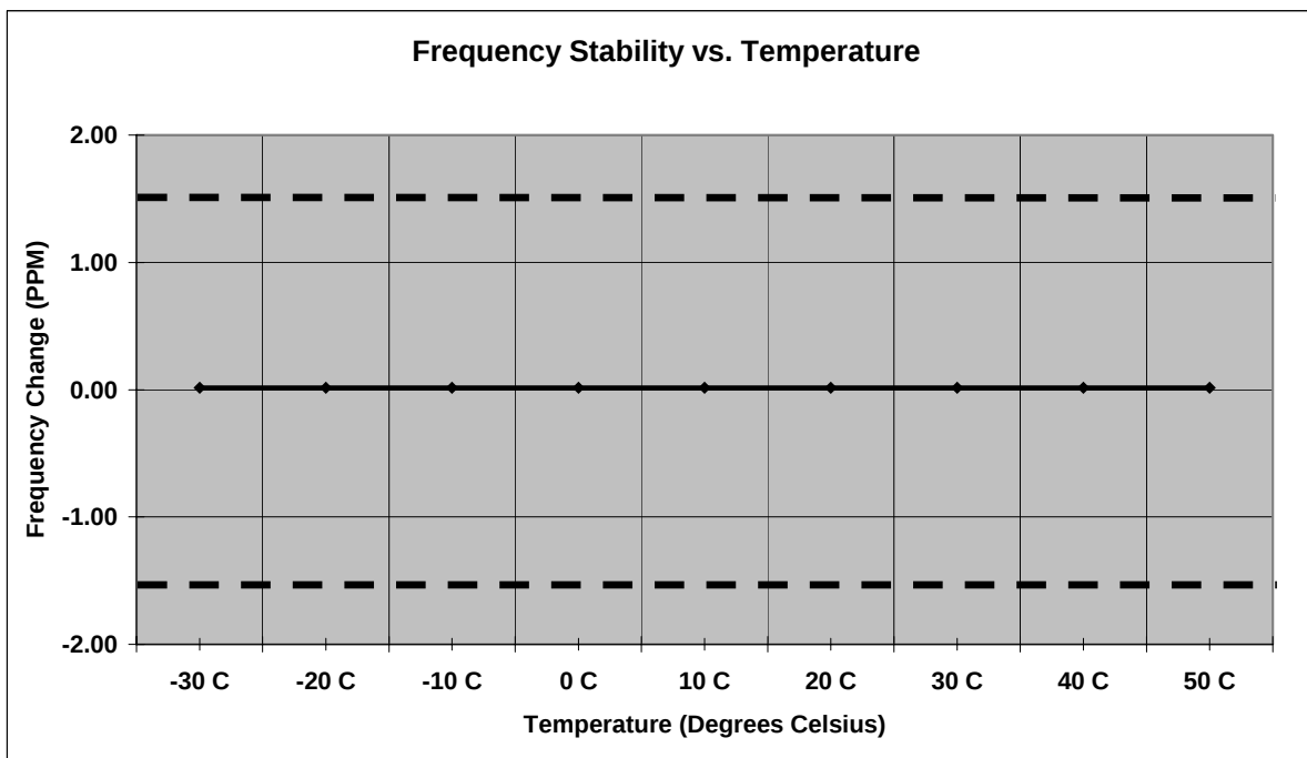
Figure 7.9-3: Frequency Stability Uplink – High Channel
