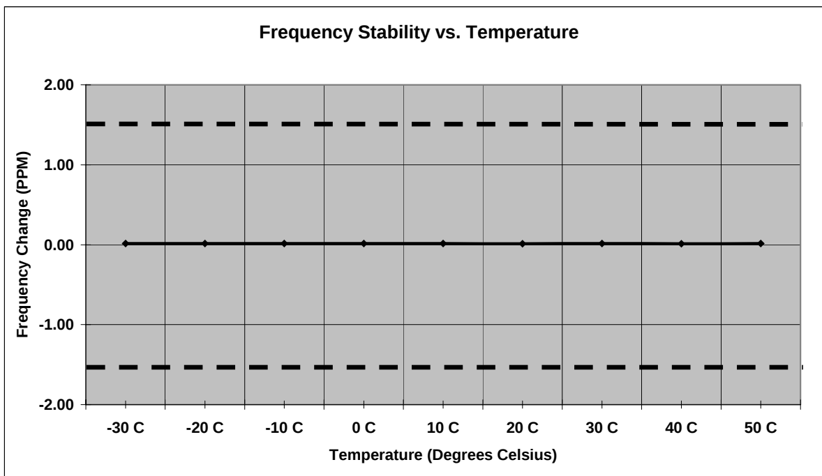
Figure 7.9-6: Frequency Stability Downlink – High Channel
