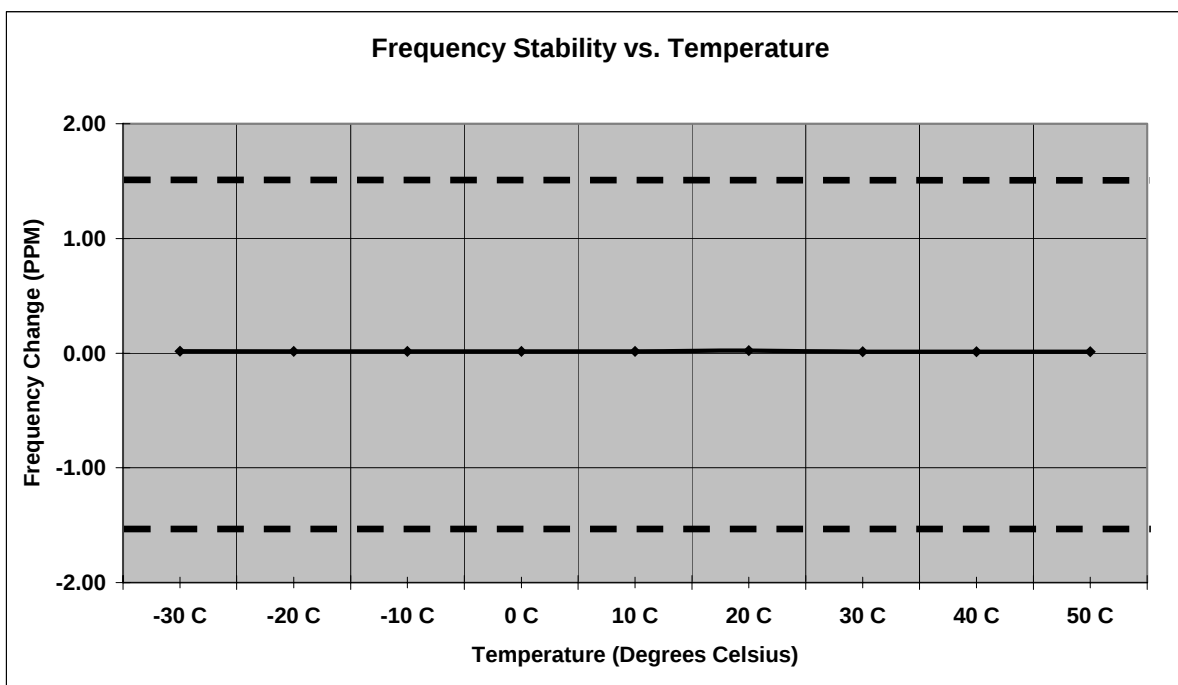
Figure 7.9-5: Frequency Stability Downlink – Middle Channel
