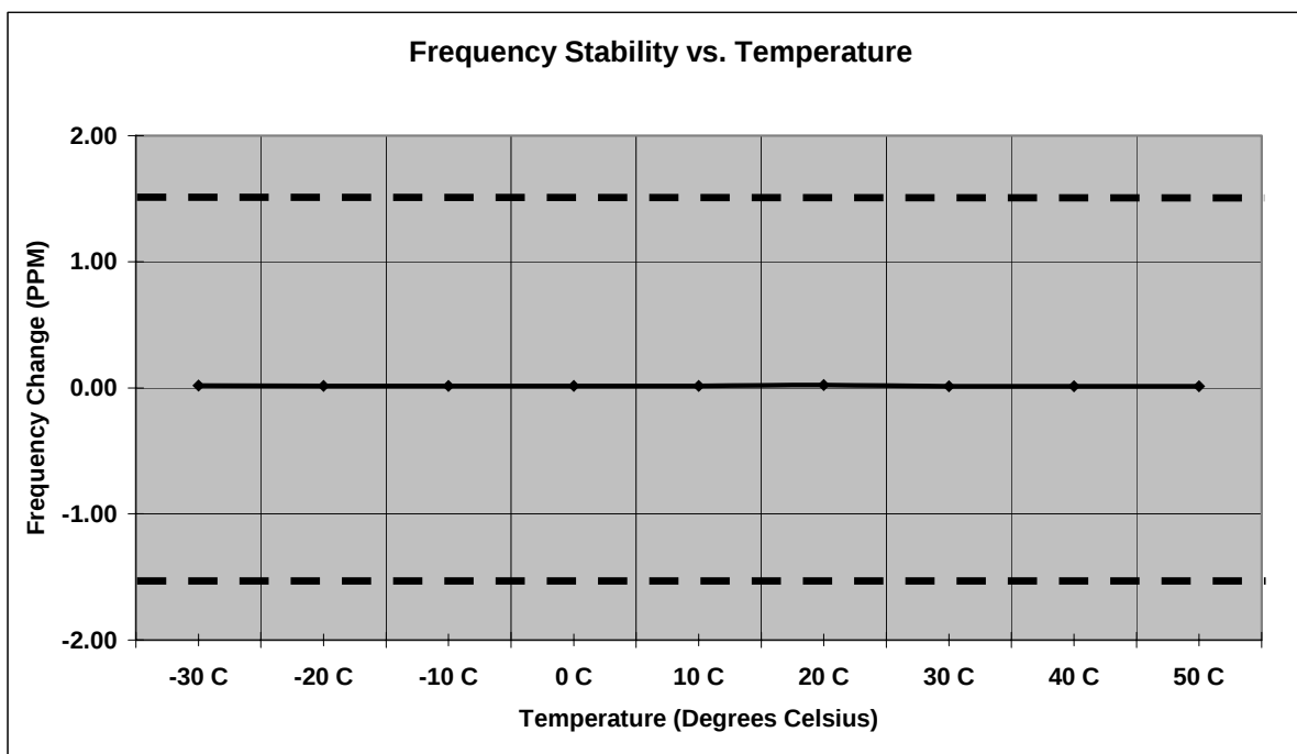
Figure 7.9-4: Frequency Stability Downlink – Low Channel
