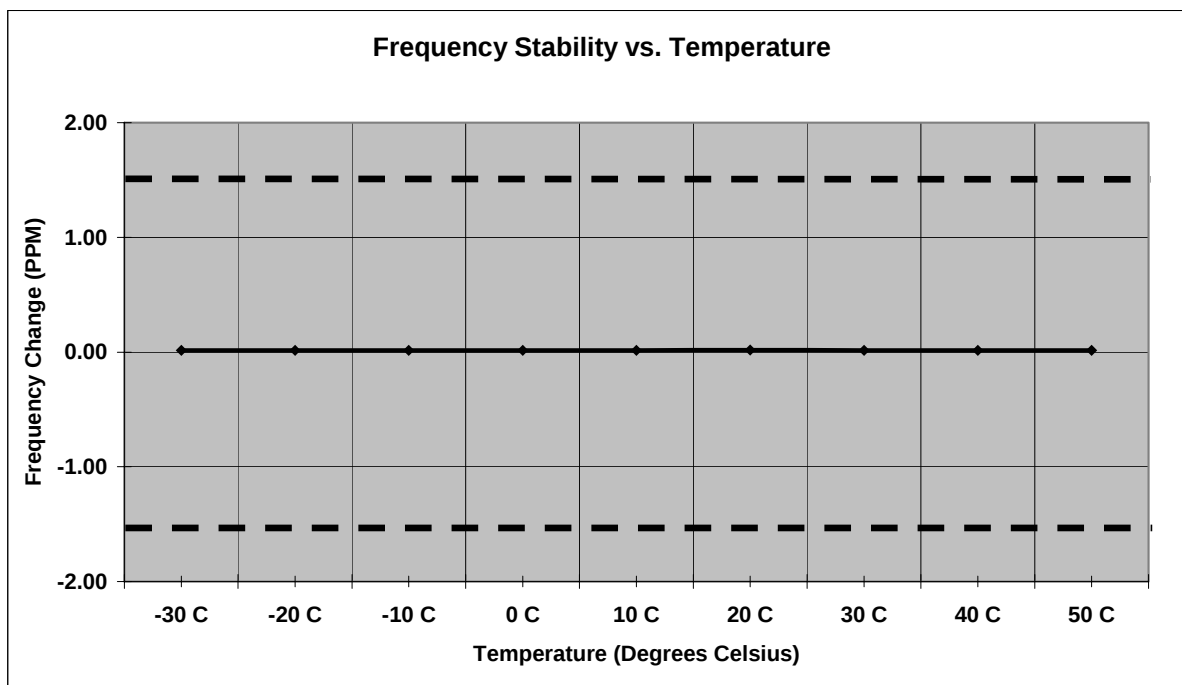
Figure 7.9-2: Frequency Stability Uplink – Middle Channel
