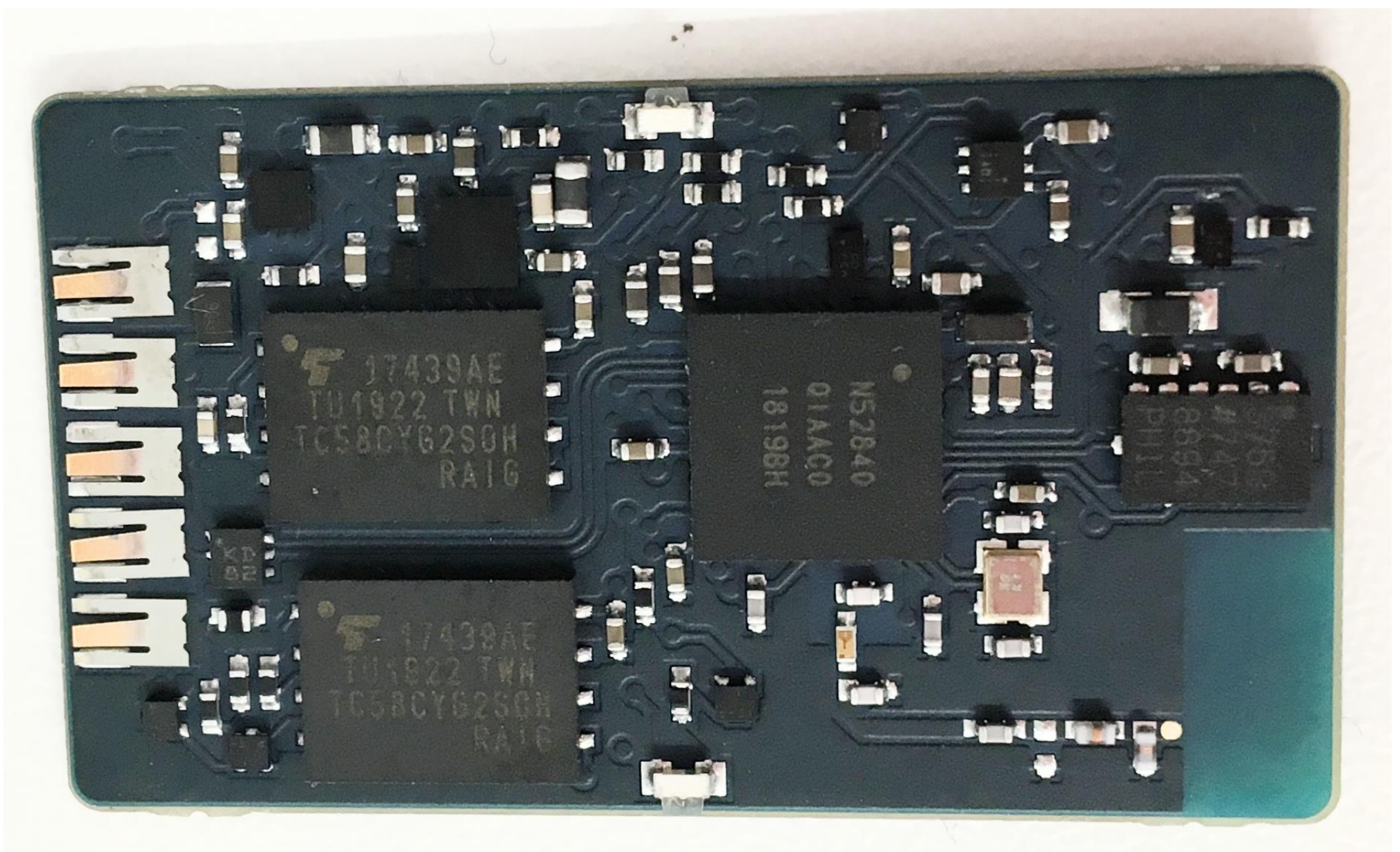
Lower PCB View
