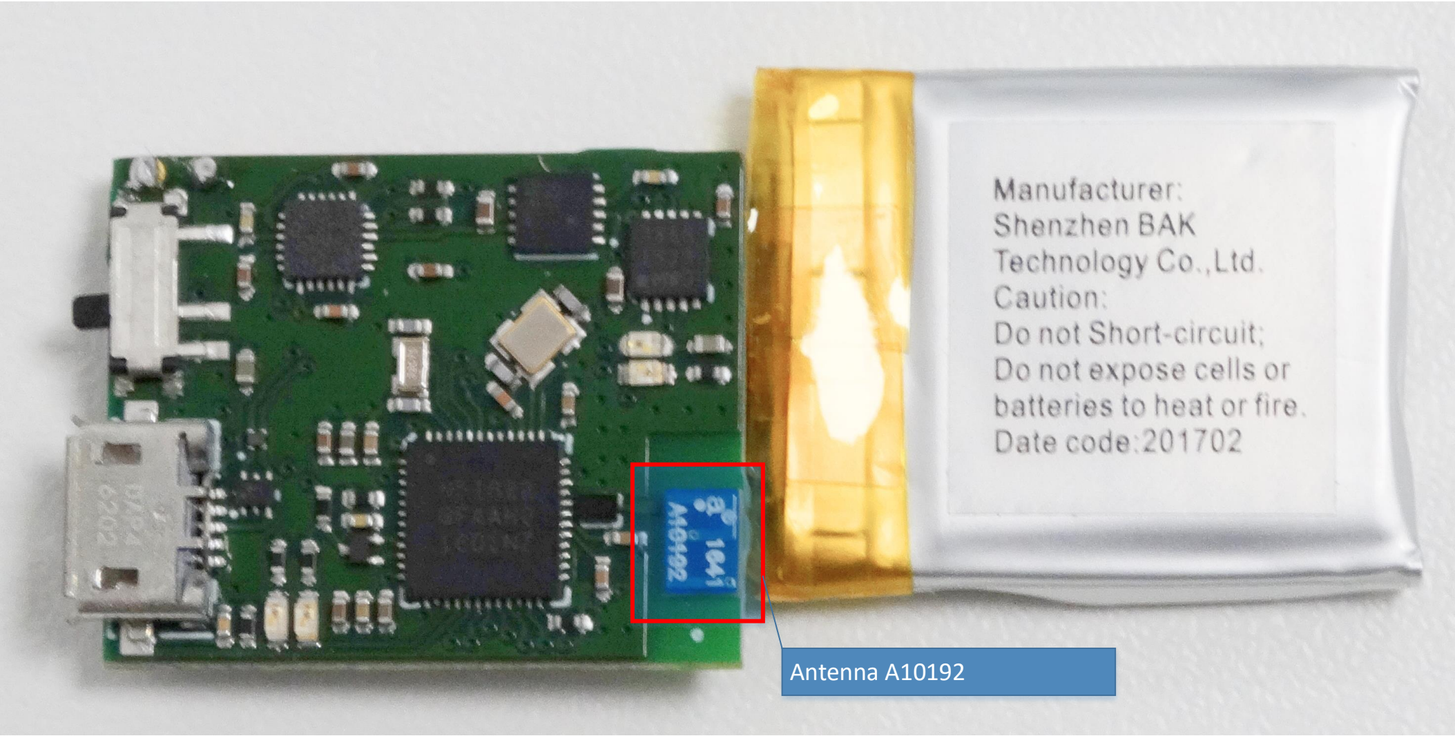
Top View and Antenna Location
