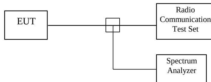
Figure 2 : Modulation characteristic measurement configuration
