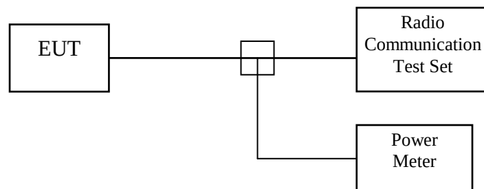
Figure 1: Transmit power measurement configuration.
