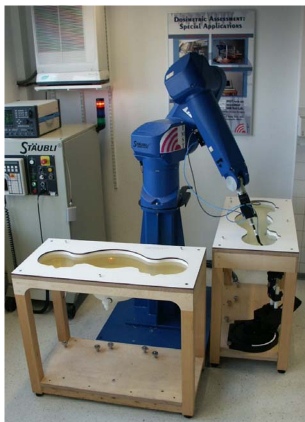
Fig. 7: The measurement set-up with two SAM phantoms containing tissue simulating liquid.
