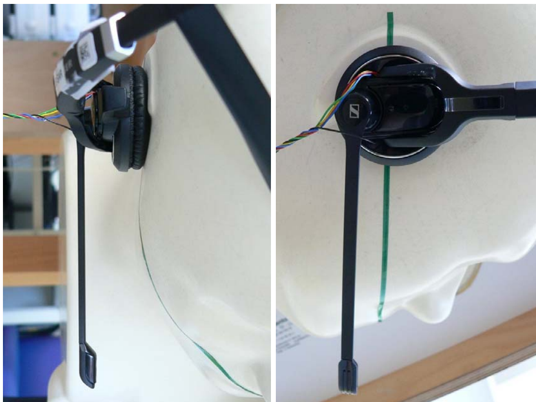
Fig. 14: Cheek position, right side, antenna 1 and 2.
