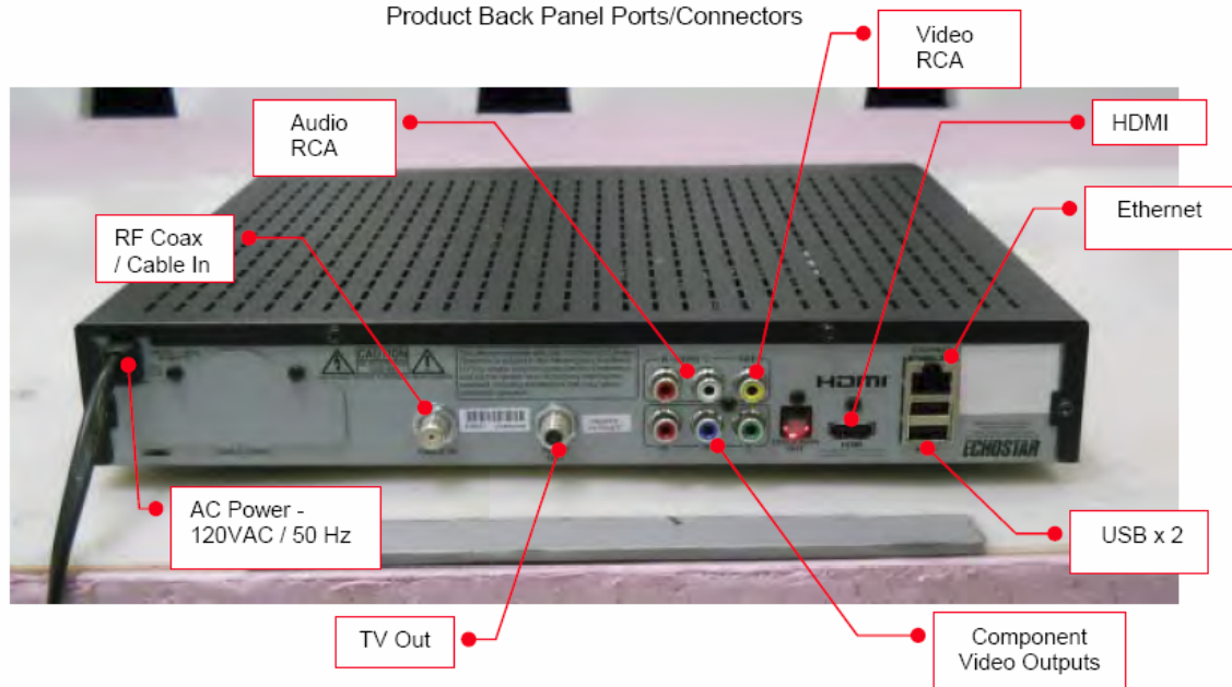
Product Back Panel Ports/Connectors
