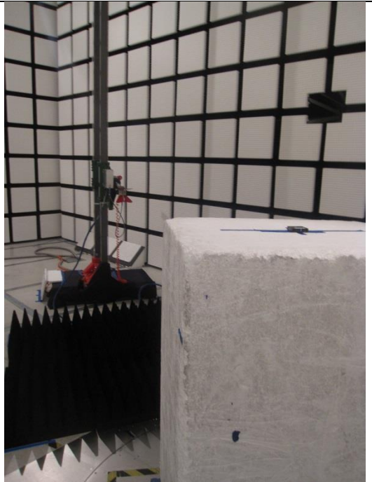
RADIATED BACK PHOTO (ABOVE 1 GHz)
