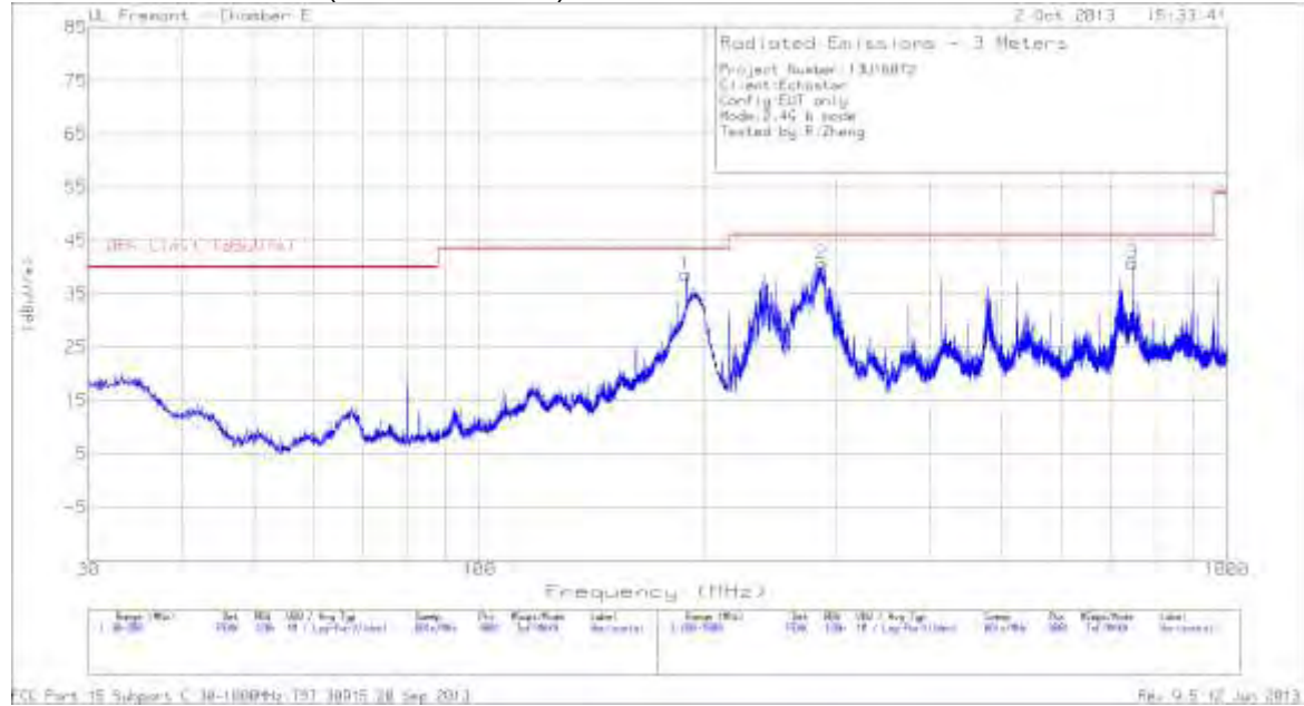
HORIZONTAL PLOT (2.4 GHz BAND)
