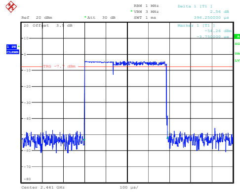
2DH1_Hopping 0.396ms
