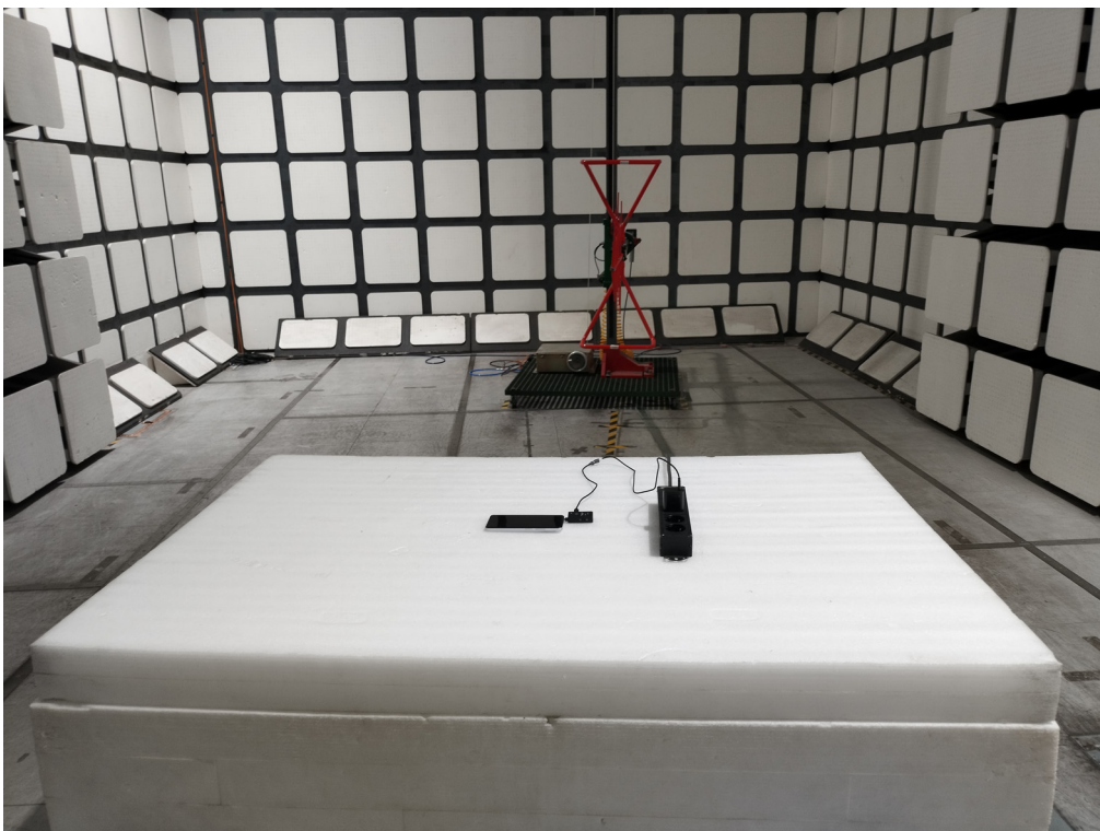
Radiated Emissions View (30 MHz- 1 GHz)
