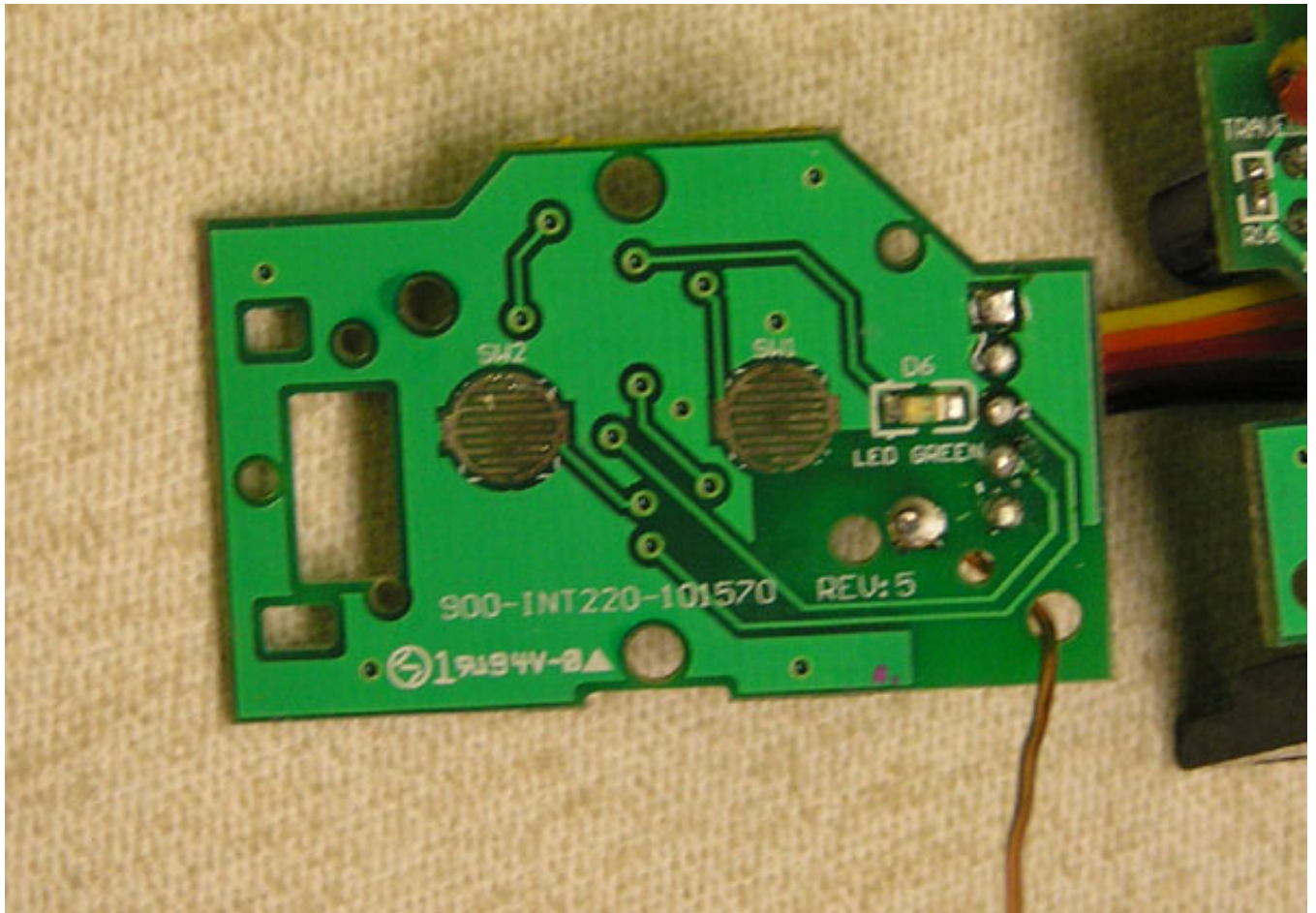
HA20 KEY PCB TOP
