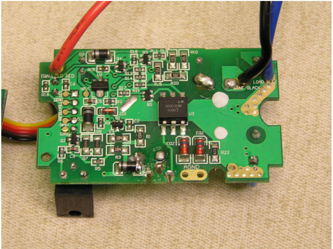
HA20 POWER PCB BOTTOM
