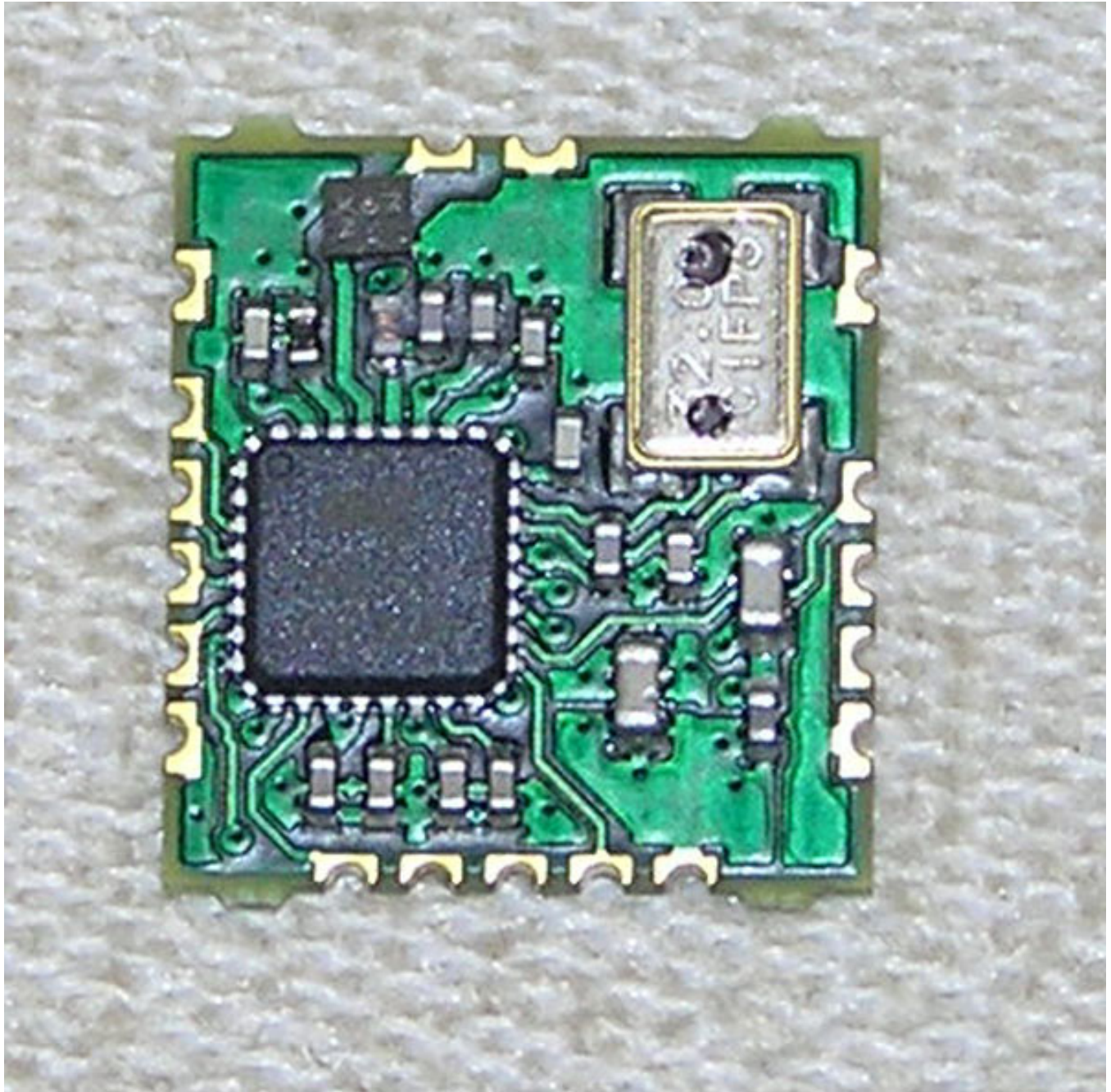
HA20 RF MODULE PCB ZM3102N FRONT
