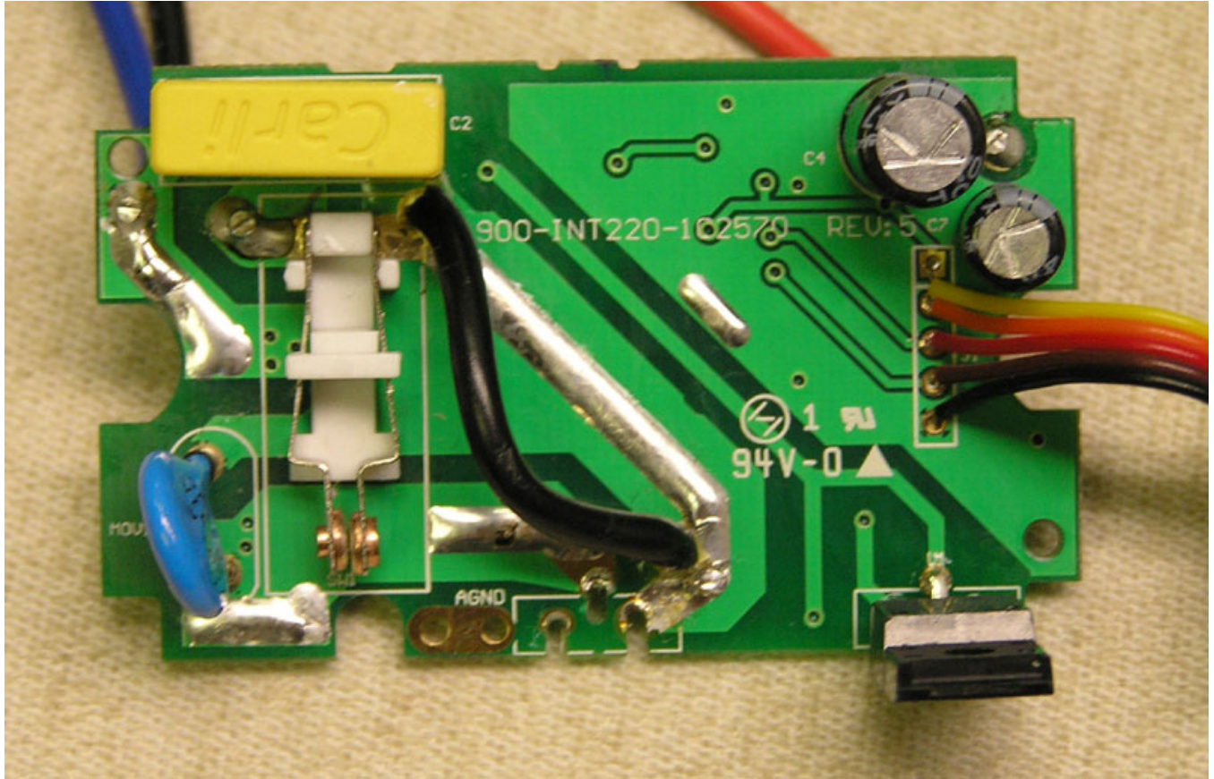
HA20 POWER PCB TOP
