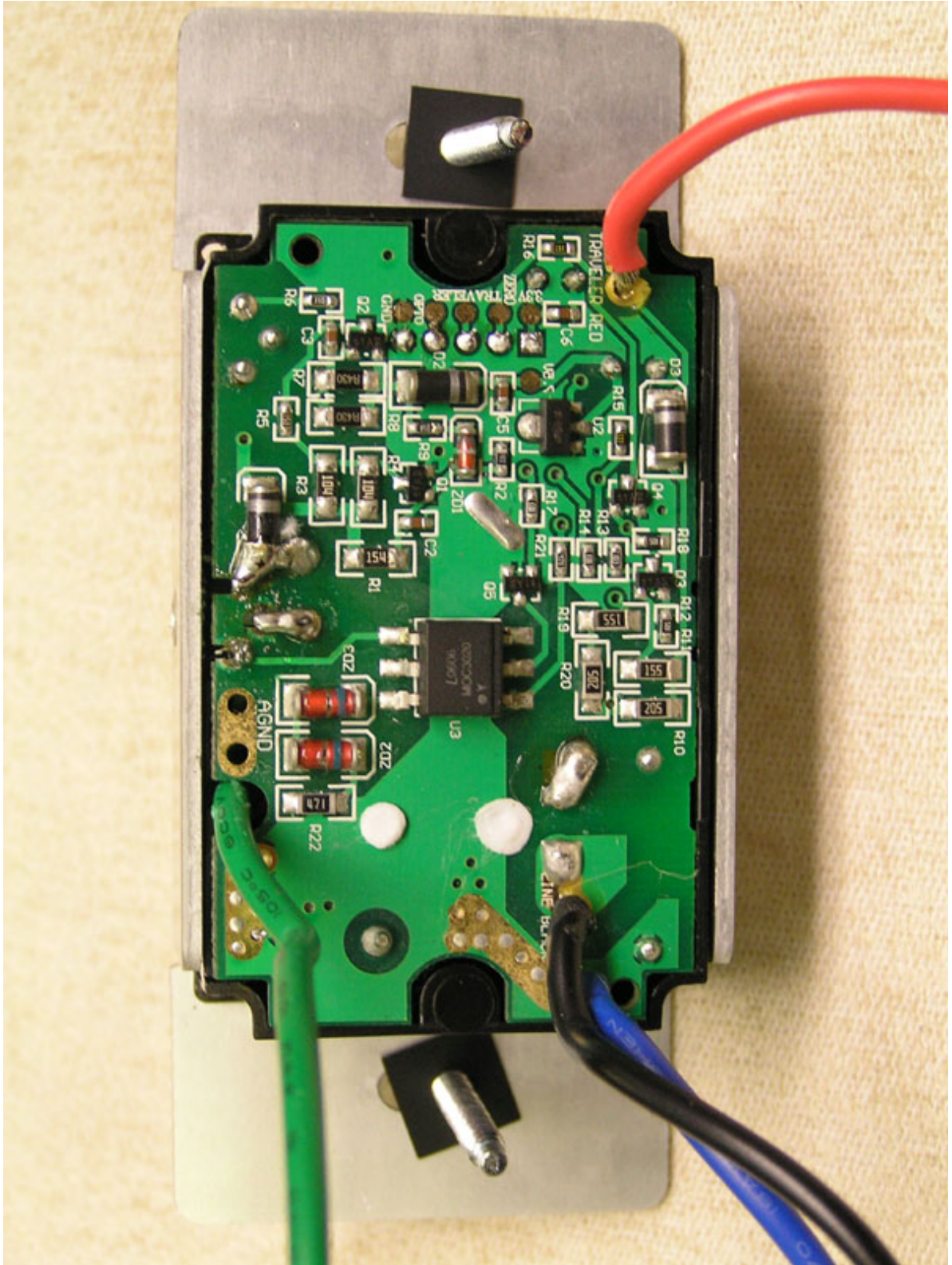
HA20 REAR PLASTIC HOUSING REMOVED
