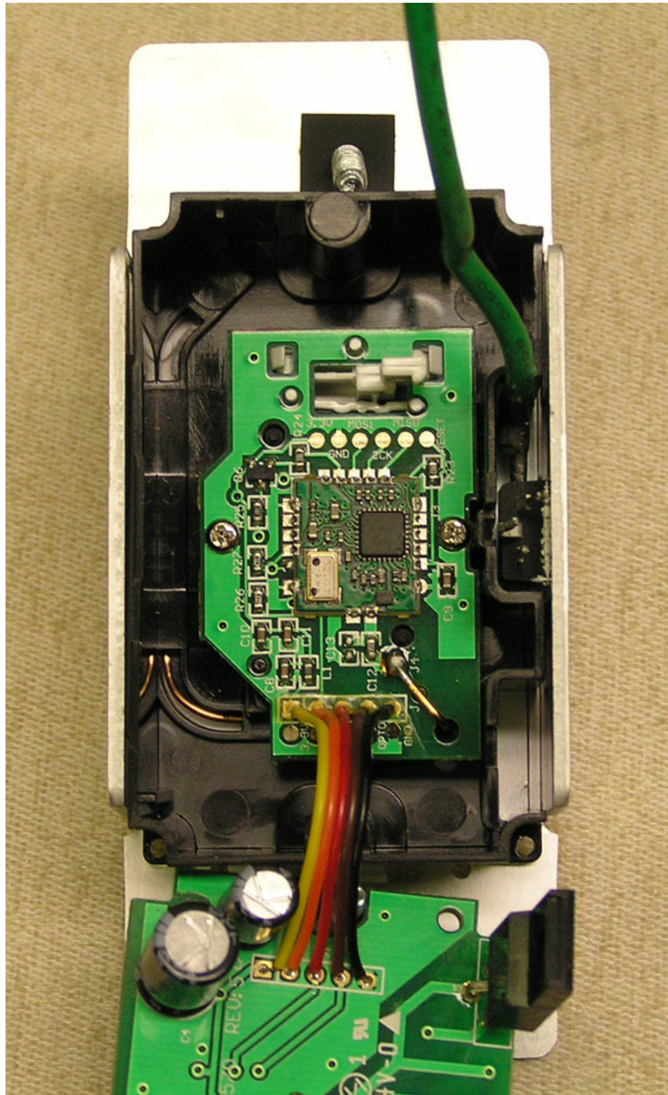
HA20 POWER PCB MOVED TO SHOW KEY PCB MOUNTED
