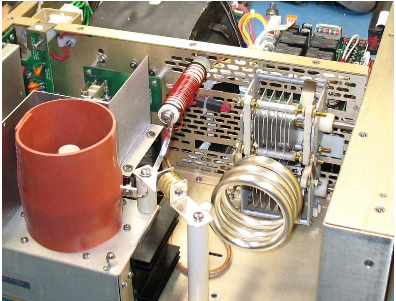
Output Tank
