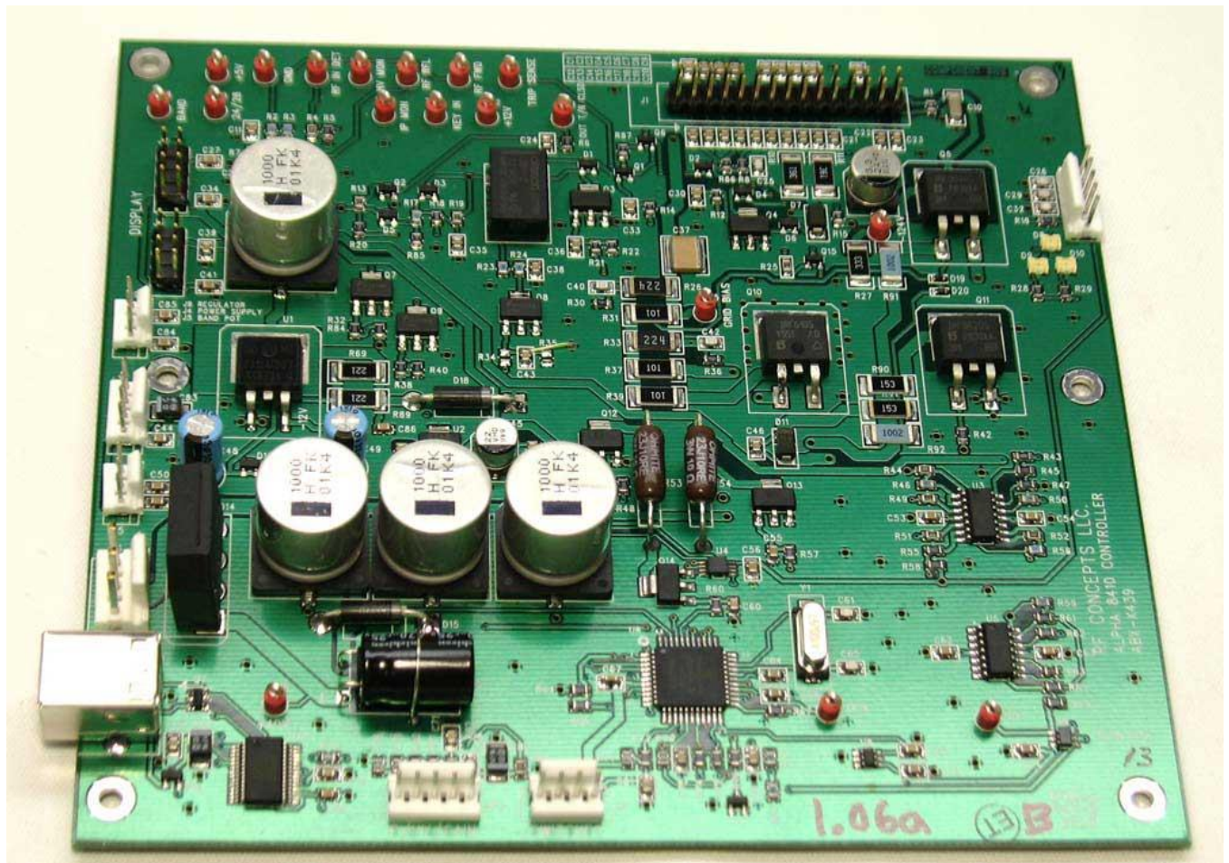
Micro Processor Board
