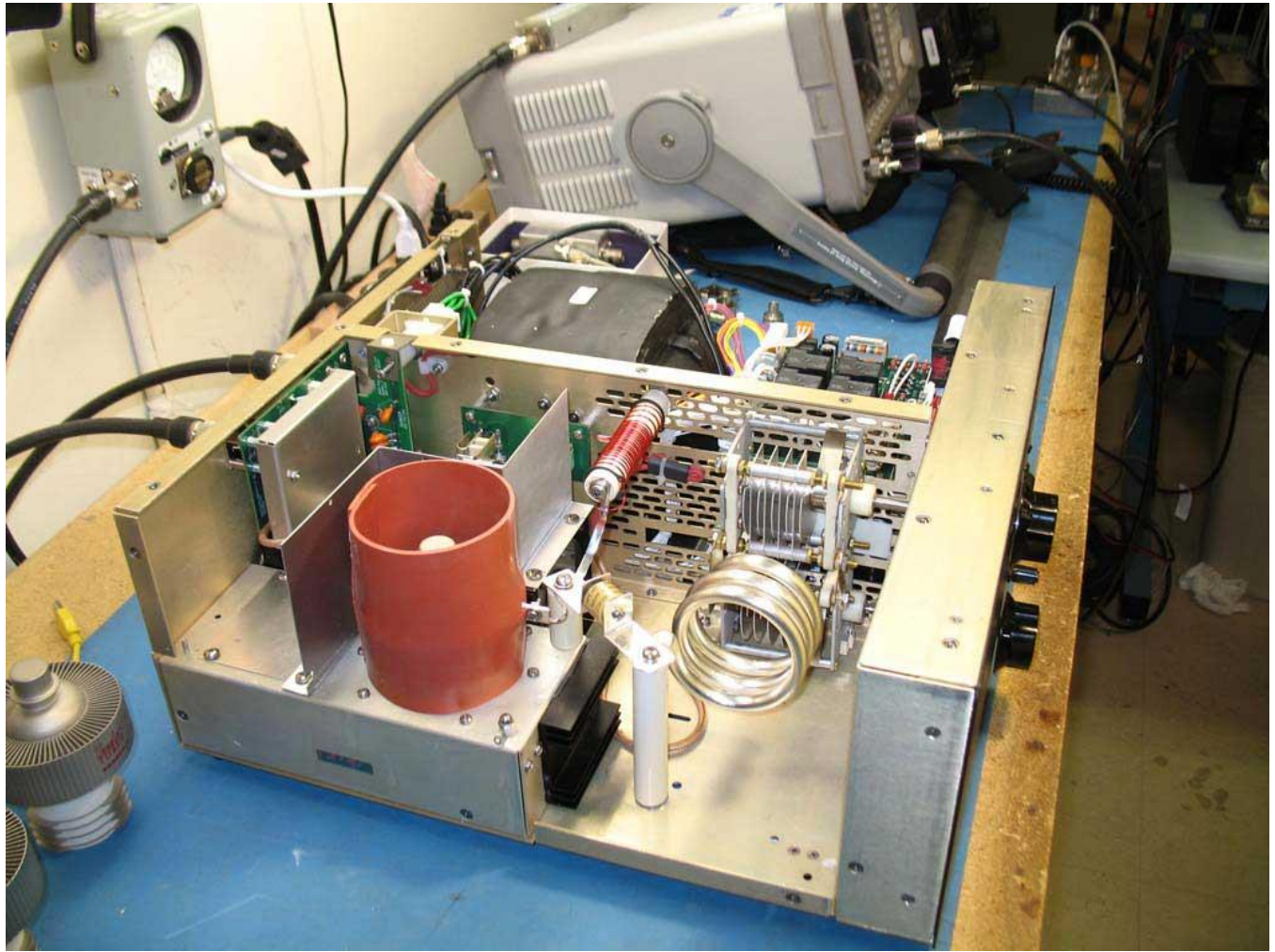
RF Tank and Tube Side of the Amplifier Left Side
