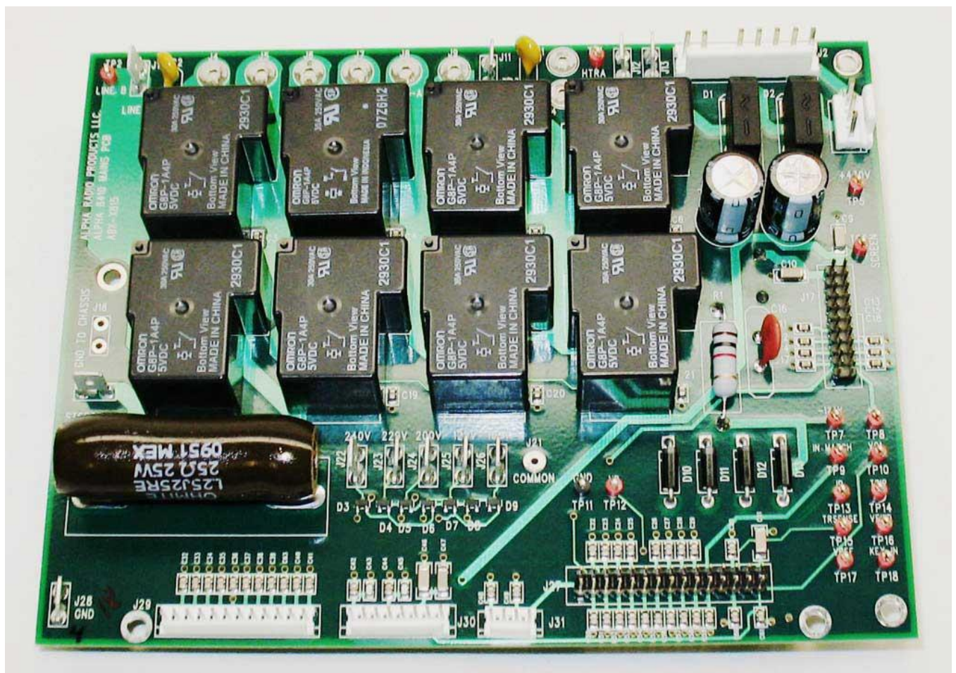
AC Relay PCB - Top
