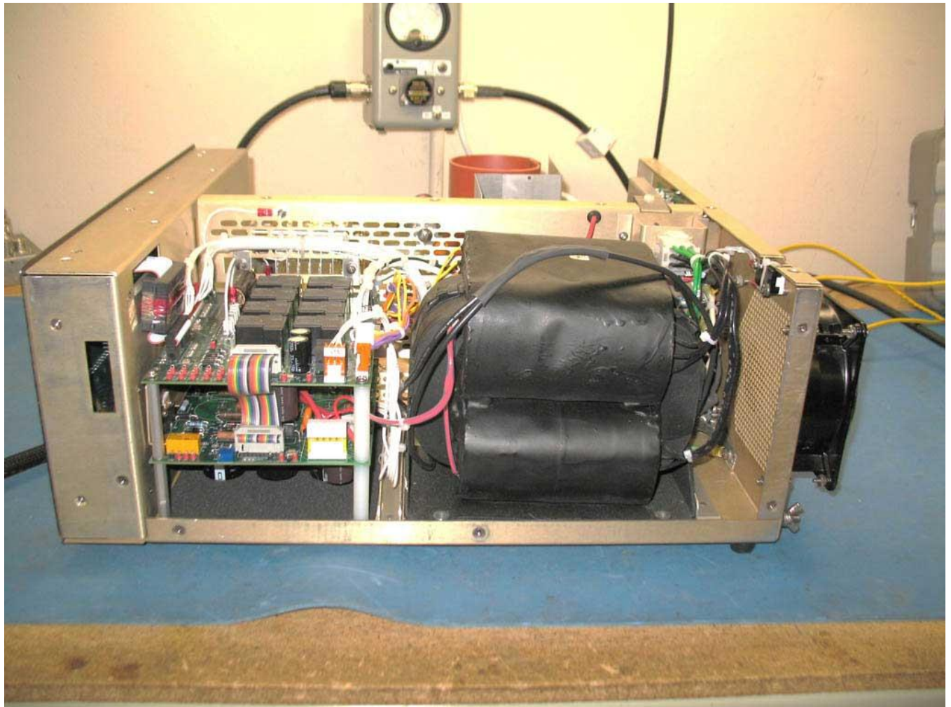
Power Supply Side of the Amplifier With Transformer Right Side.
