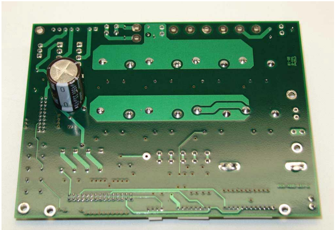
AC Relay PCB - Bottom
