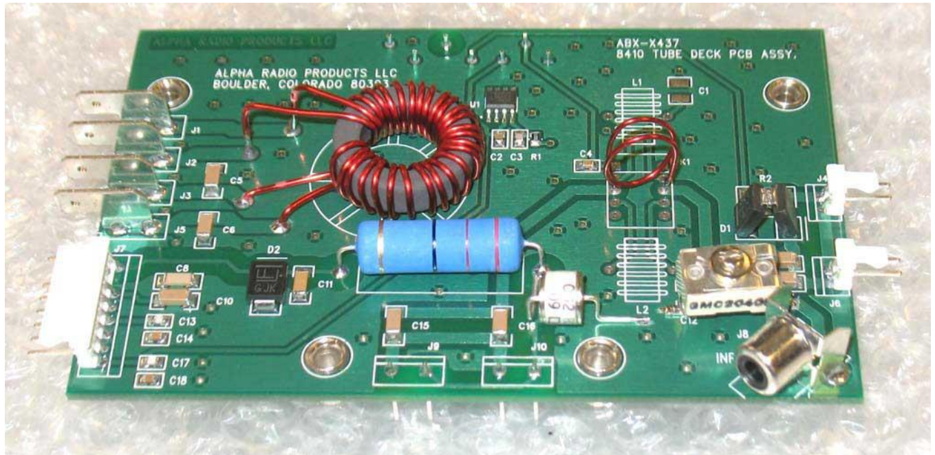
Input Filter Board
