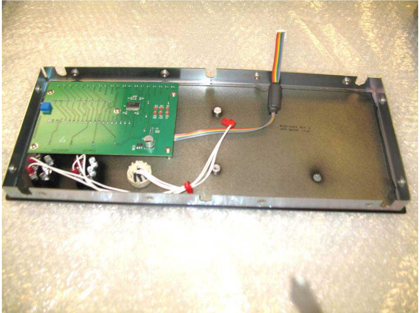
Front Panel Inside View
