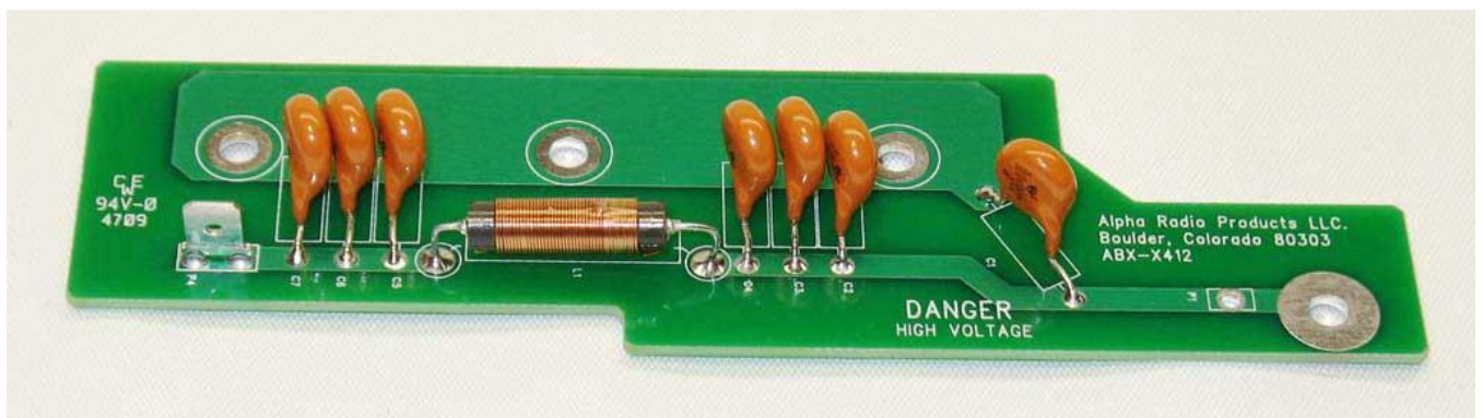
High Voltage Filter Board
