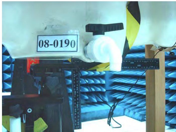
Figure 18. Body SAR Test Setup (Flat Section) _ 15 mm separation
