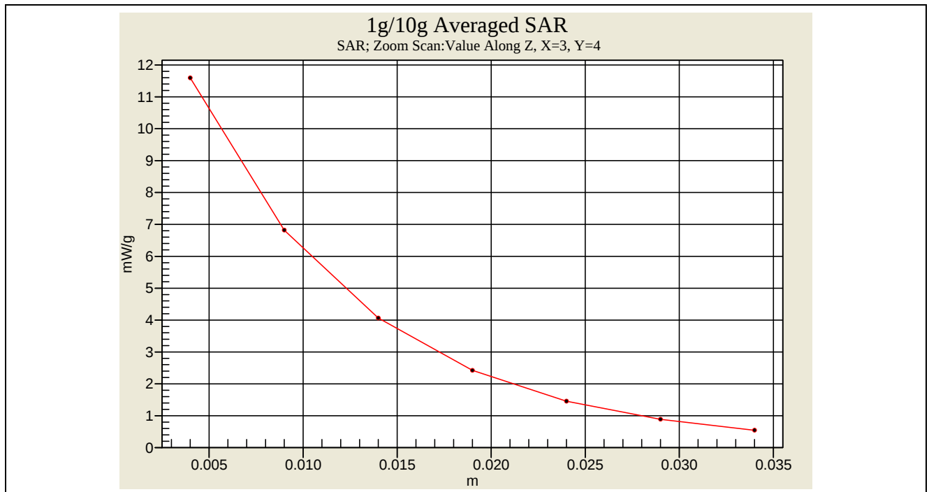
Body-Tissue-Simulating-Liquid 1950MHz ( 2008.07.21 )
