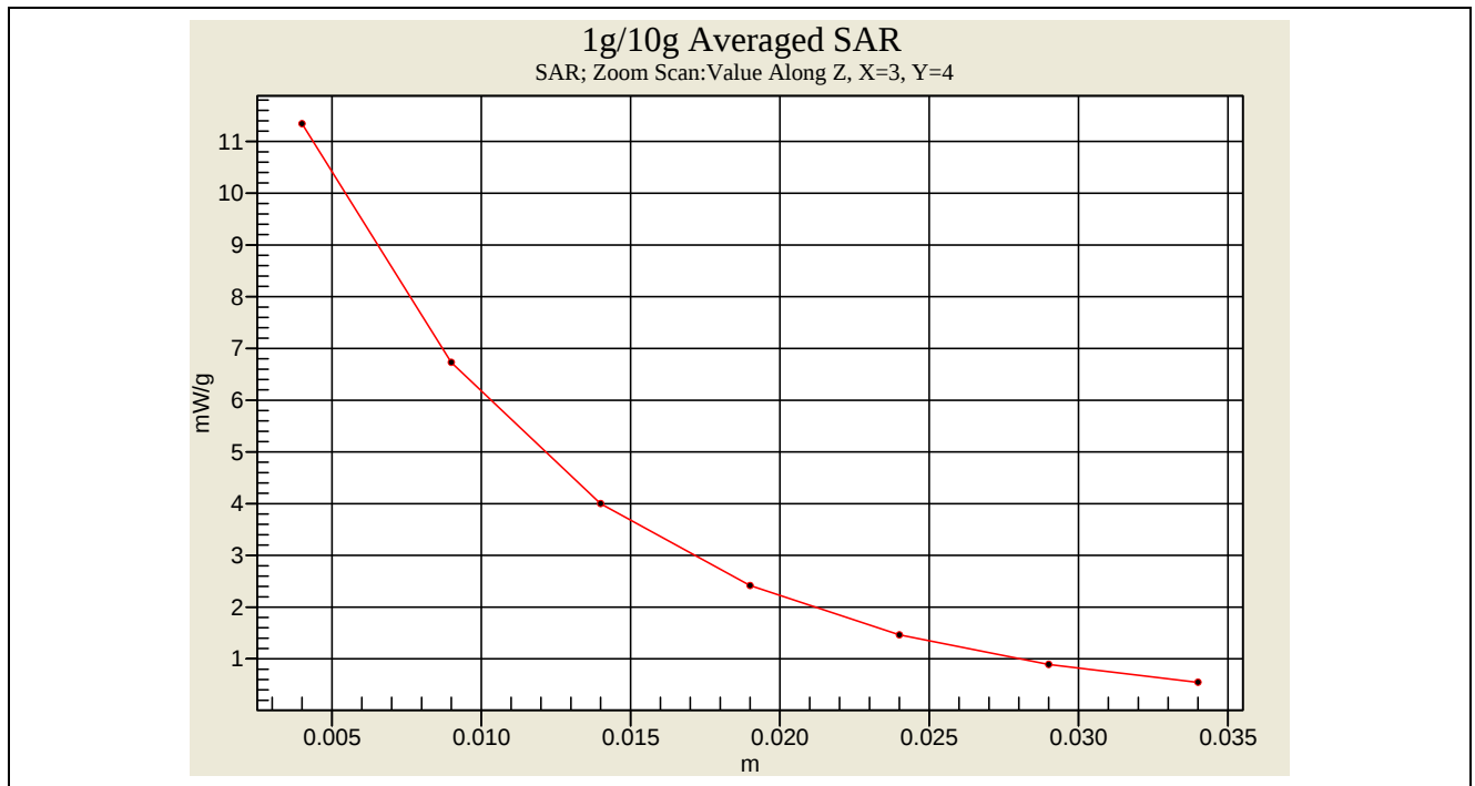
Head-Tissue-Simulating-Liquid 1950MHz ( 2008.07.17 )
