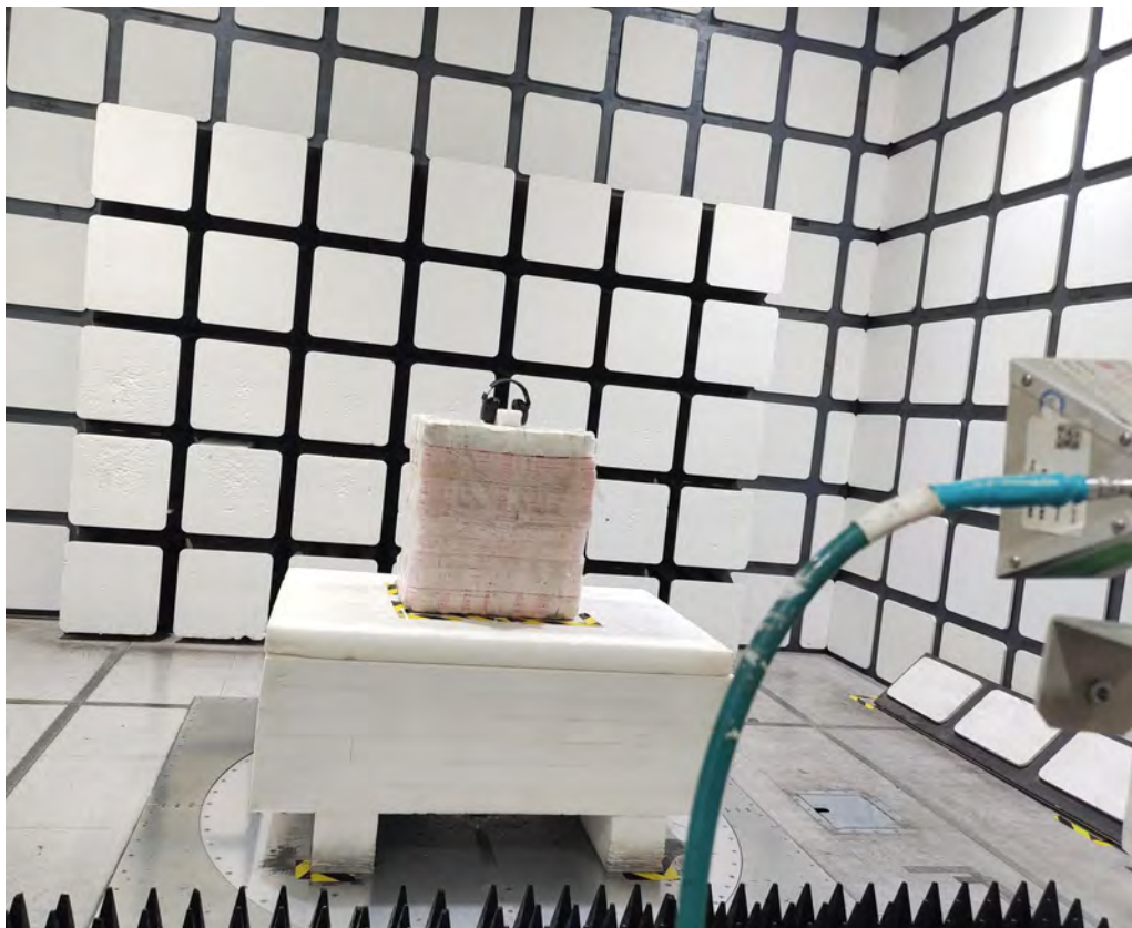
Radiated Emissions View (18-25 GHz)
