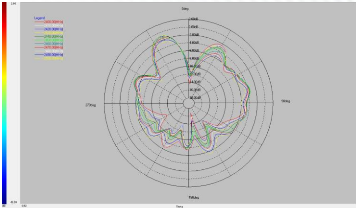
YZ plane \phi=90^\circ
