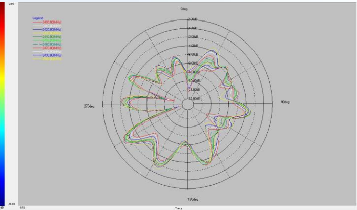
XZ plane \phi=0^\circ
