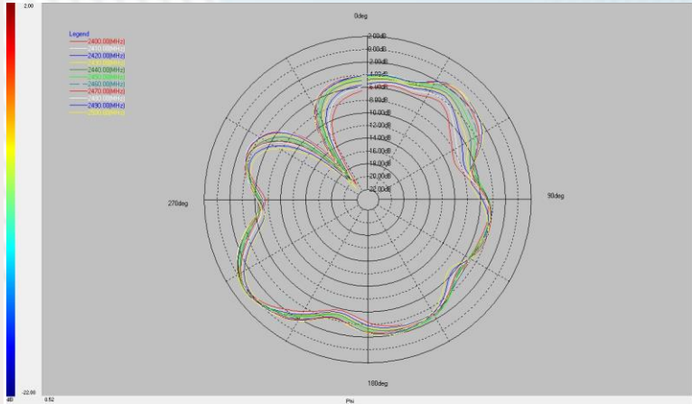
XY plane \theta=90^\circ
