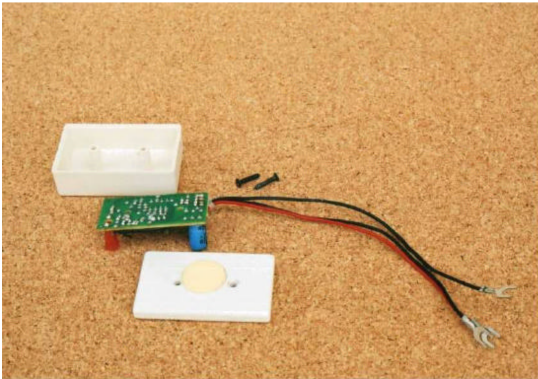
DE47DC3500T Transmitter Open - Top
