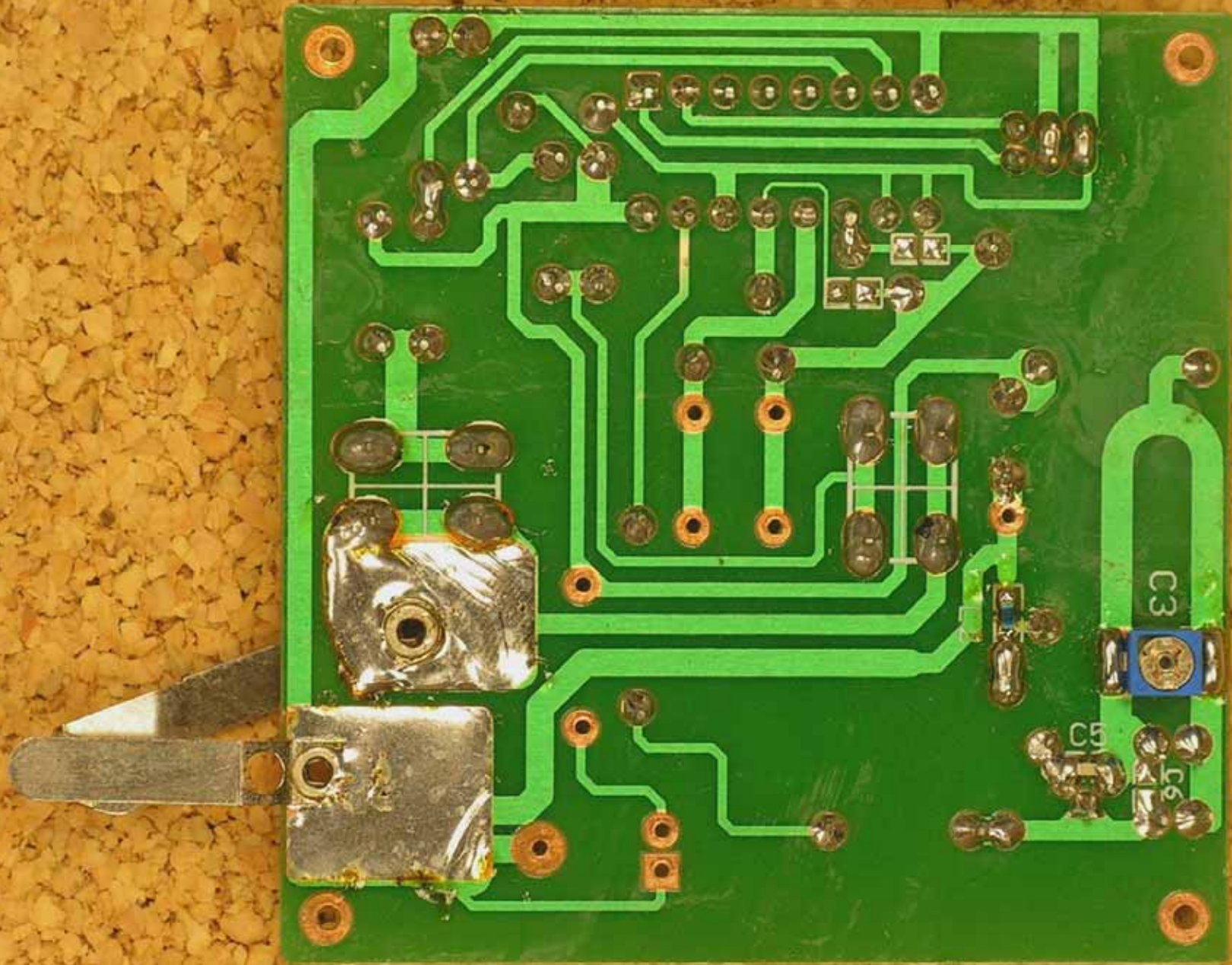
PCB (bottom)
