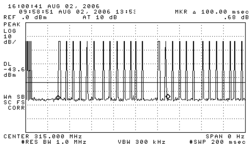
Figure 6.1(b). Transmissions modulation characteristics: (top) wake wide pulse, (center) wake narrow pulse, (bottom) PPM data.
