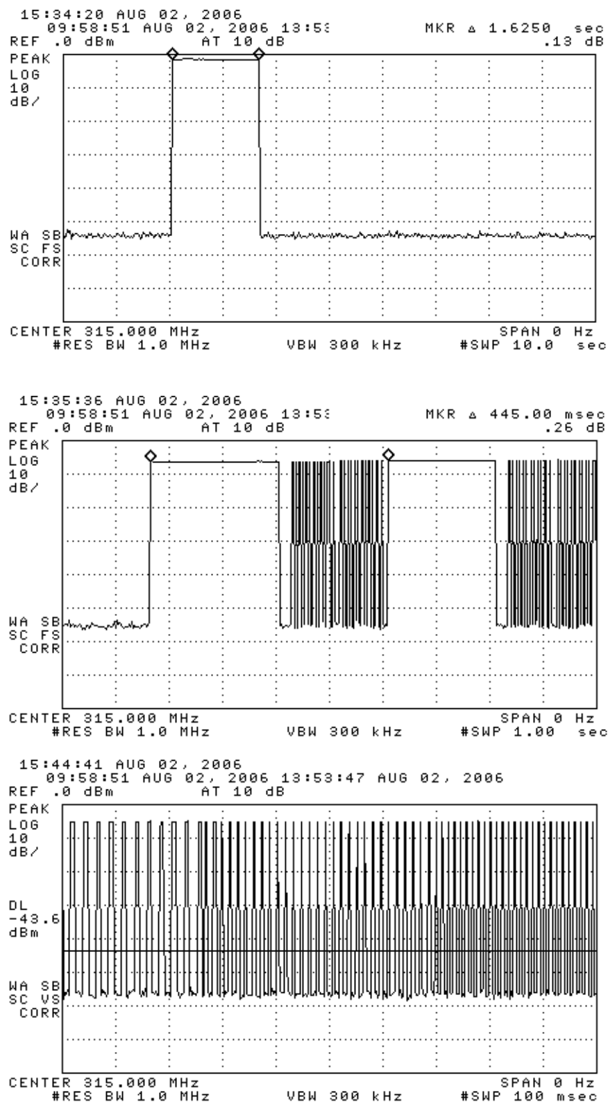
Figure 6.1(a). Transmissions modulation characteristics: (top) complete transmission, (center) expanded word, (bottom) expanded wake-up.
