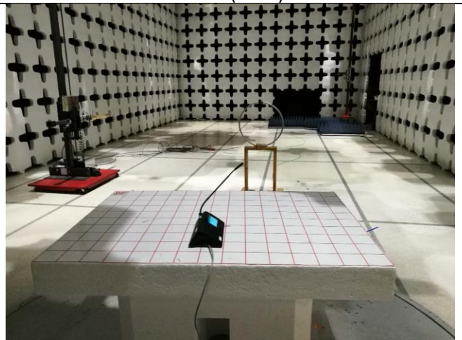
Radiated Emissions (<30MHz) 0 Degree – Rear View
