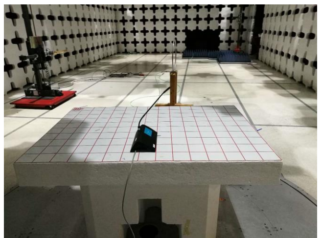
Radiated Emissions (<30MHz) 90 Degree – Rear View
