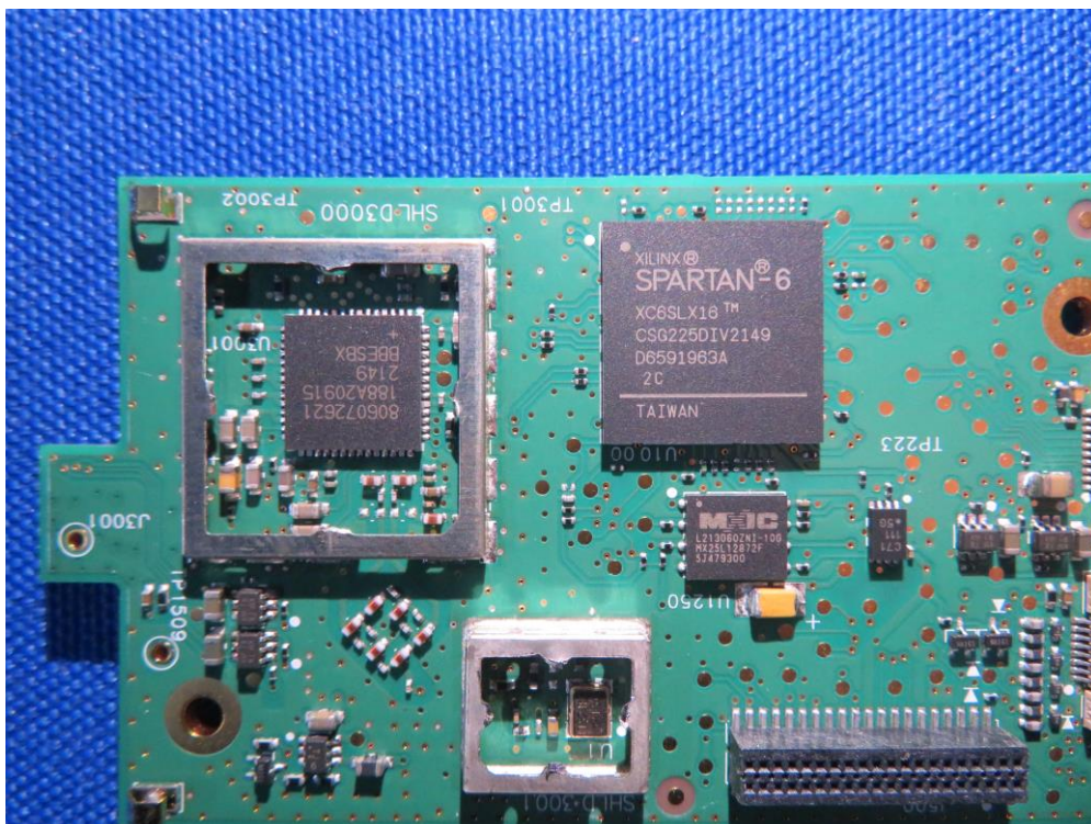
(18) EUT Photo (ADX3 G57+)
