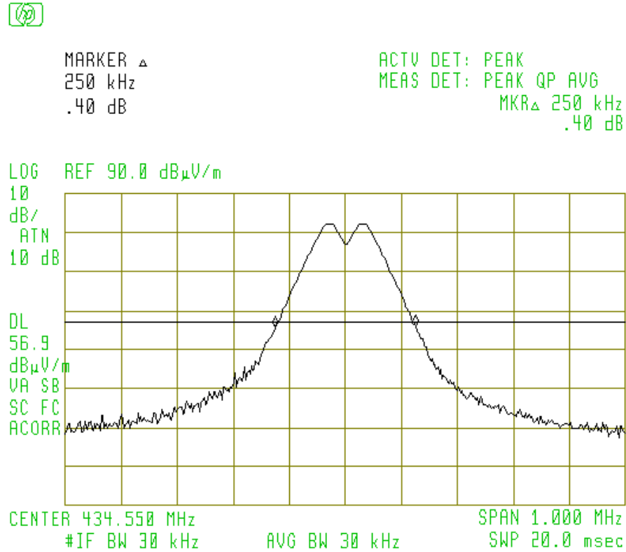
Figure 6.1 Occupied Bandwidth
