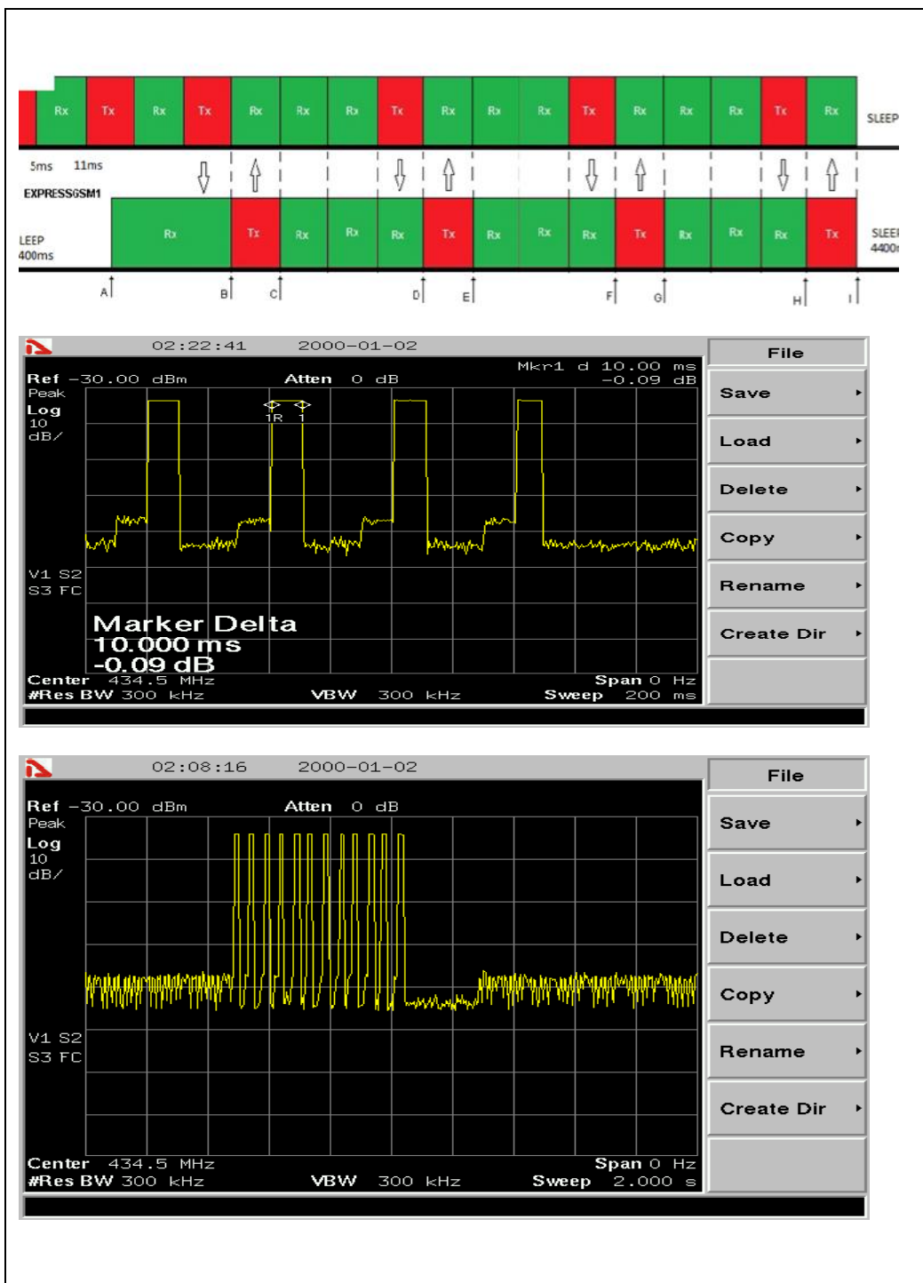
Figure 6.2 Pulse Train (w/ max. Tx duration)
