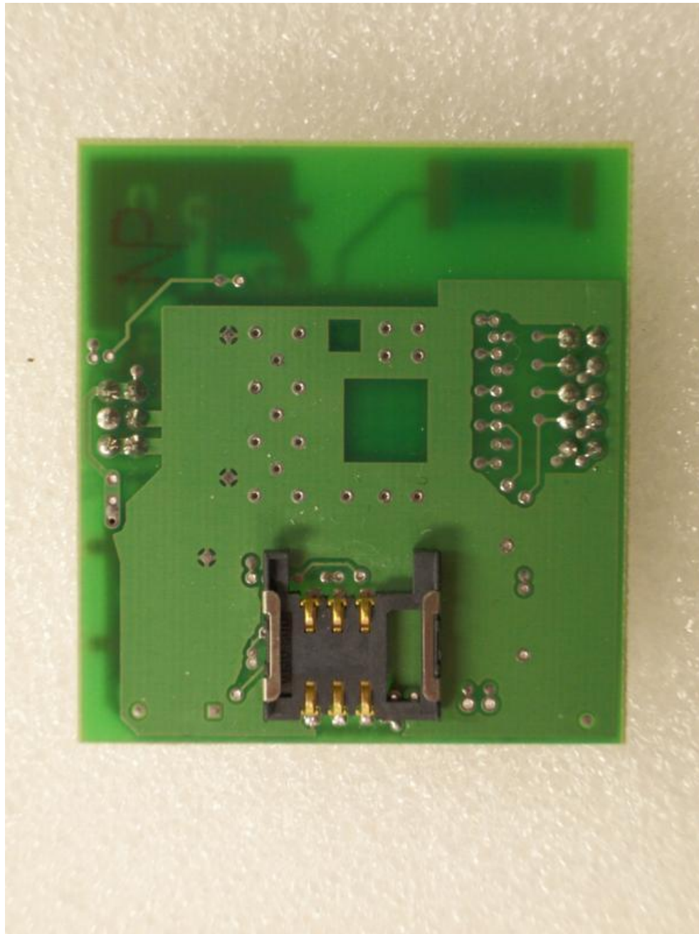
Figure 7.7 GSM Module Board Foil Side
