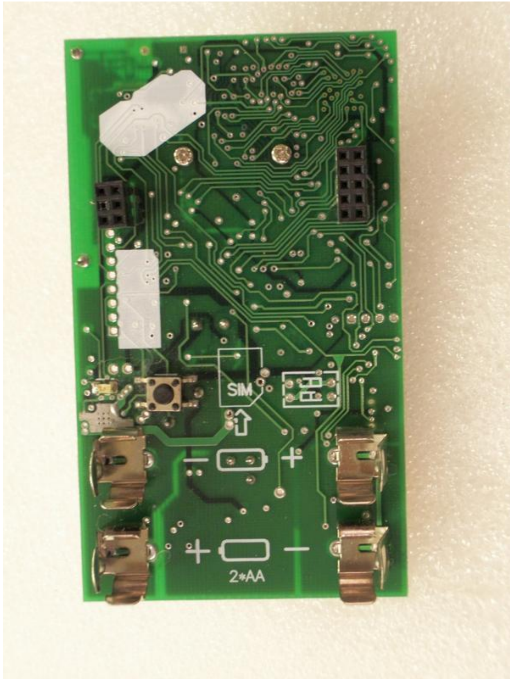
Figure 7.5 Main Board Foil Side
