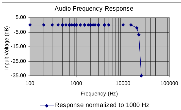
Figure 1 Audio Frequency Response Characteristics.
