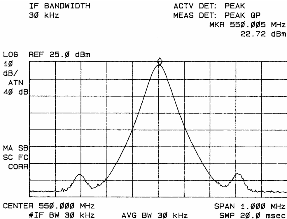
Figure 6 emissions mask
