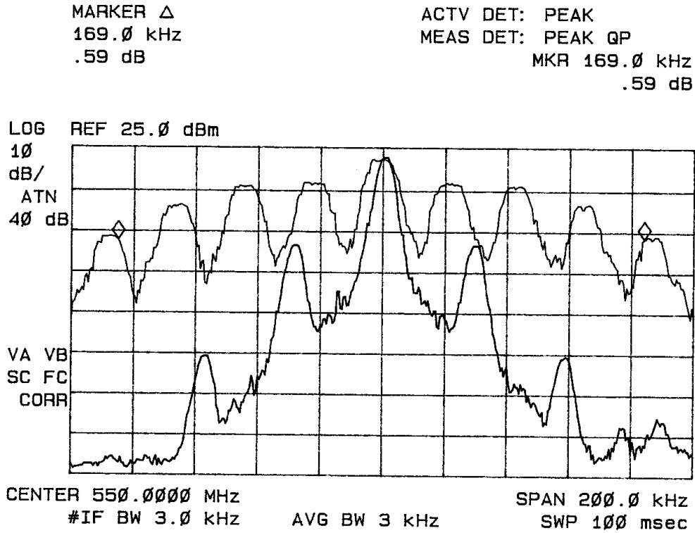
Figure 5 Occupied Bandwidth Measurement with 21,000 Hz input
