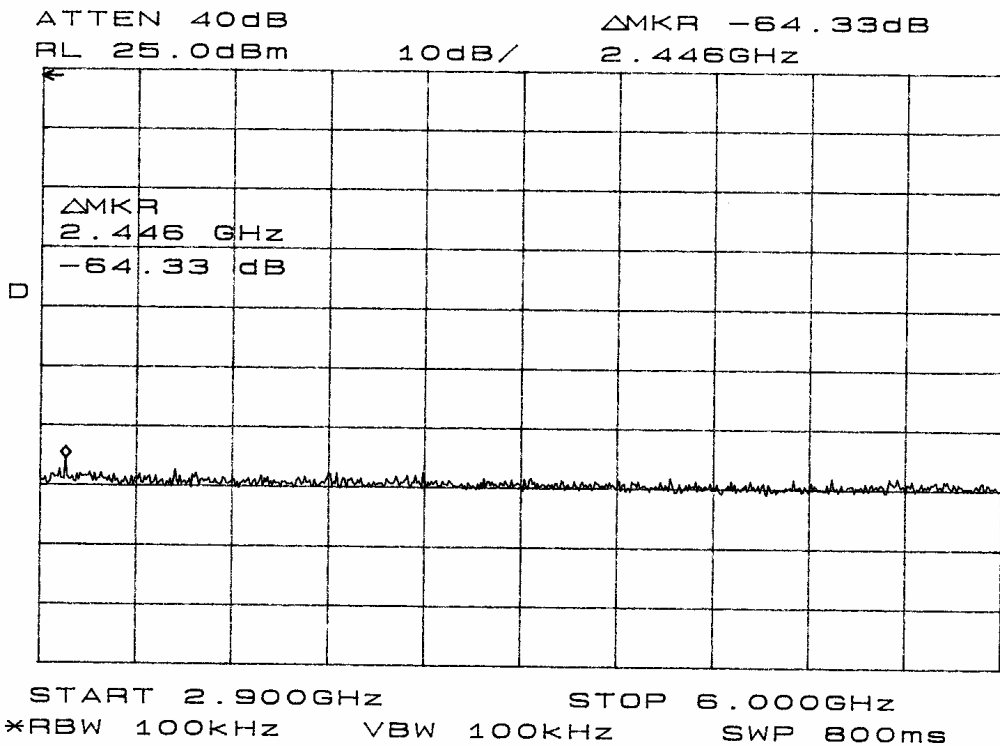
Figure 8 emissions mask
