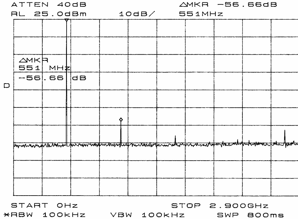
Figure 7 emissions mask
