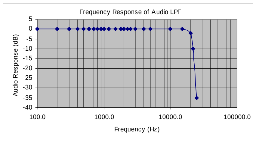
Figure 3 Frequency Response of Audio low Pass Filter.
