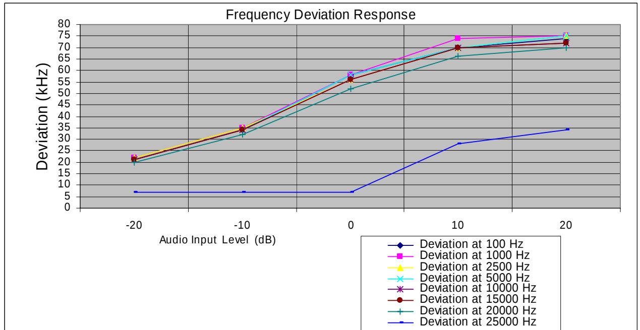
Figure 2 Deviation Characteristics.
