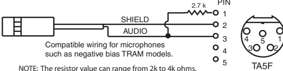
Fig. 5 - Sanken COS-11 and others
