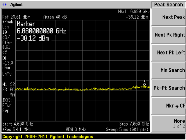
4 GHz – 7 GHz
