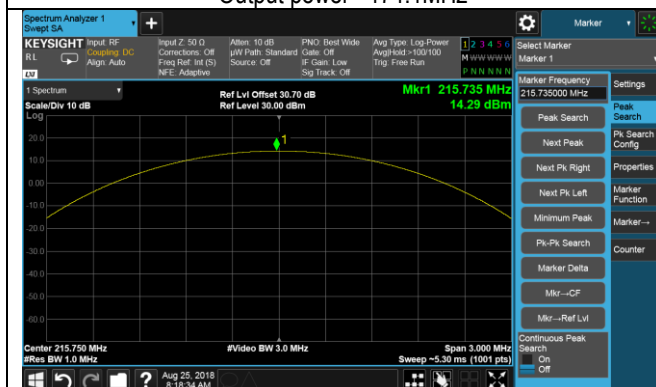
Output power - 215.75MHz
