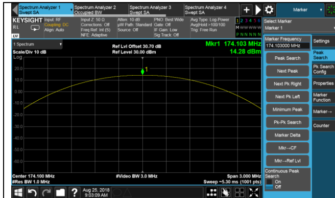
Output power –174.1MHz
