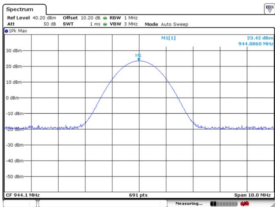
IFBT4 944.1 MHz Output Power
