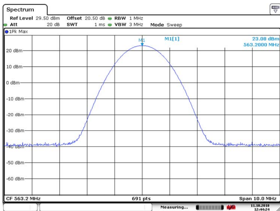
IFBT4 563.2 MHz Output Power
