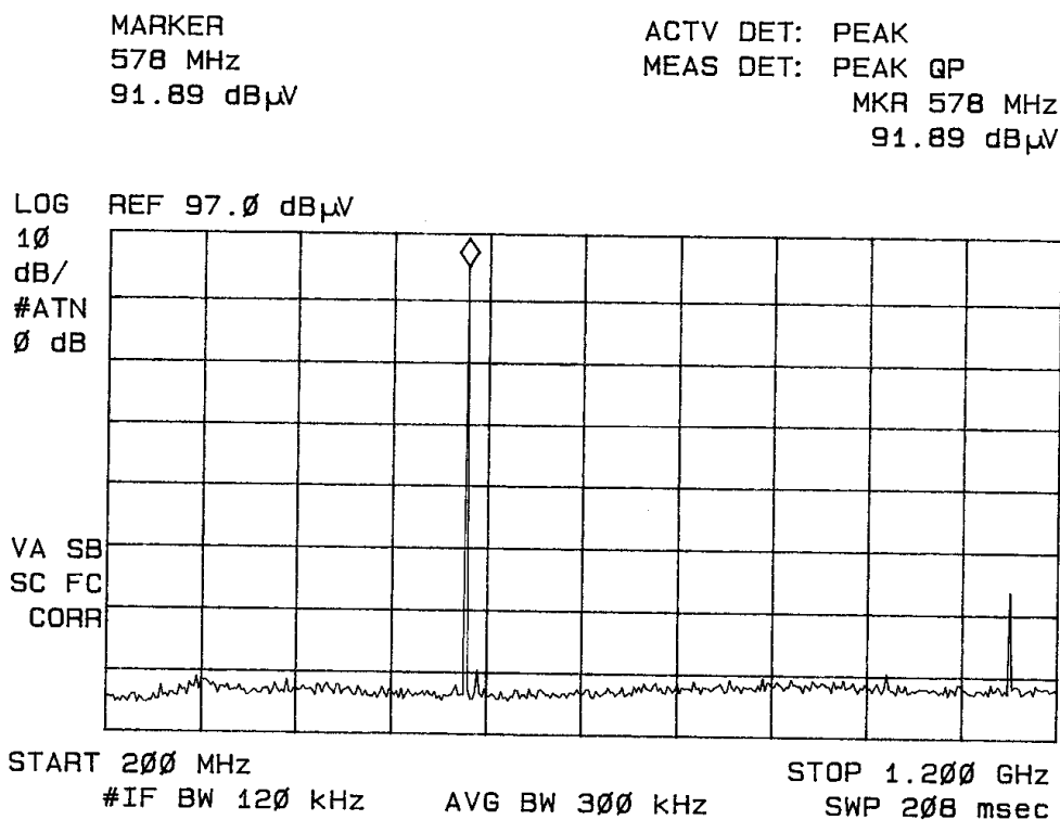
Figure seven radiated emissions
