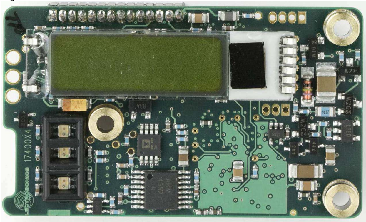
Digital PCB Back
