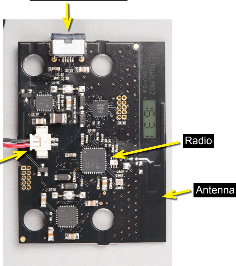
Audio/Charger Input
