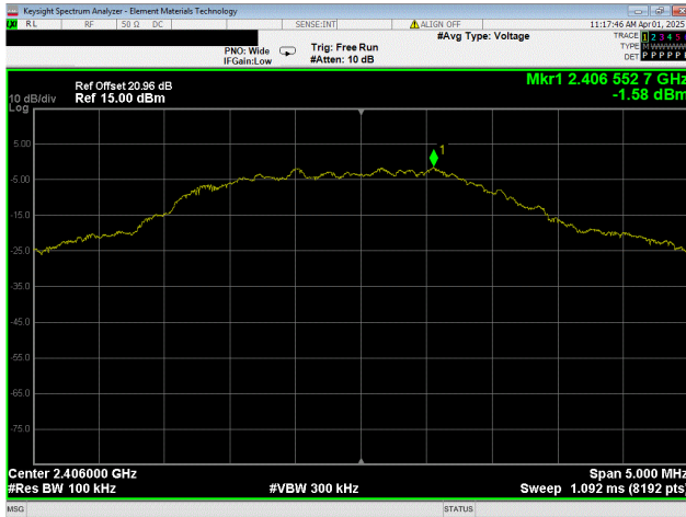
8FSK, 5Mbps Low Channel, 2406 MHz
