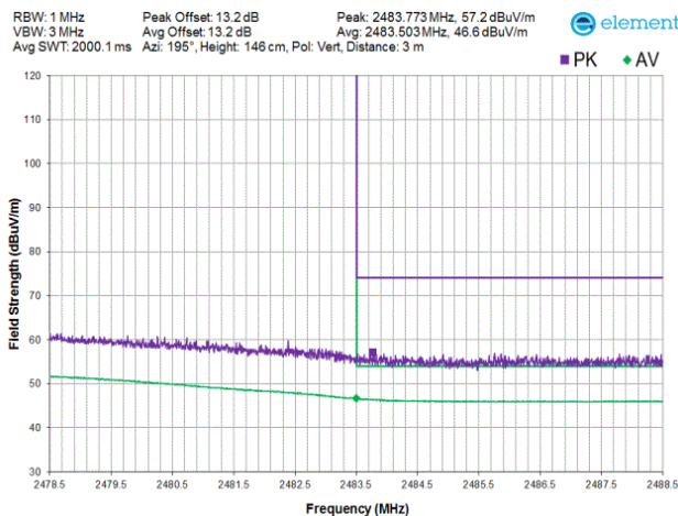
8FSK 5 Mbps High Channel, 2474 MHz EUT on Side, RX Vertical
