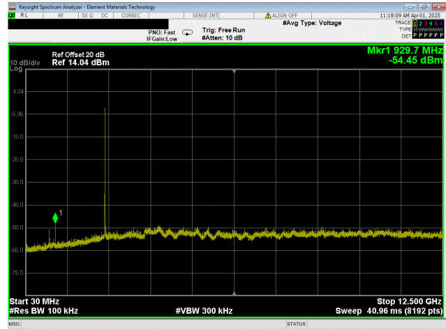
8FSK, 5Mbps Low Channel, 2406 MHz
