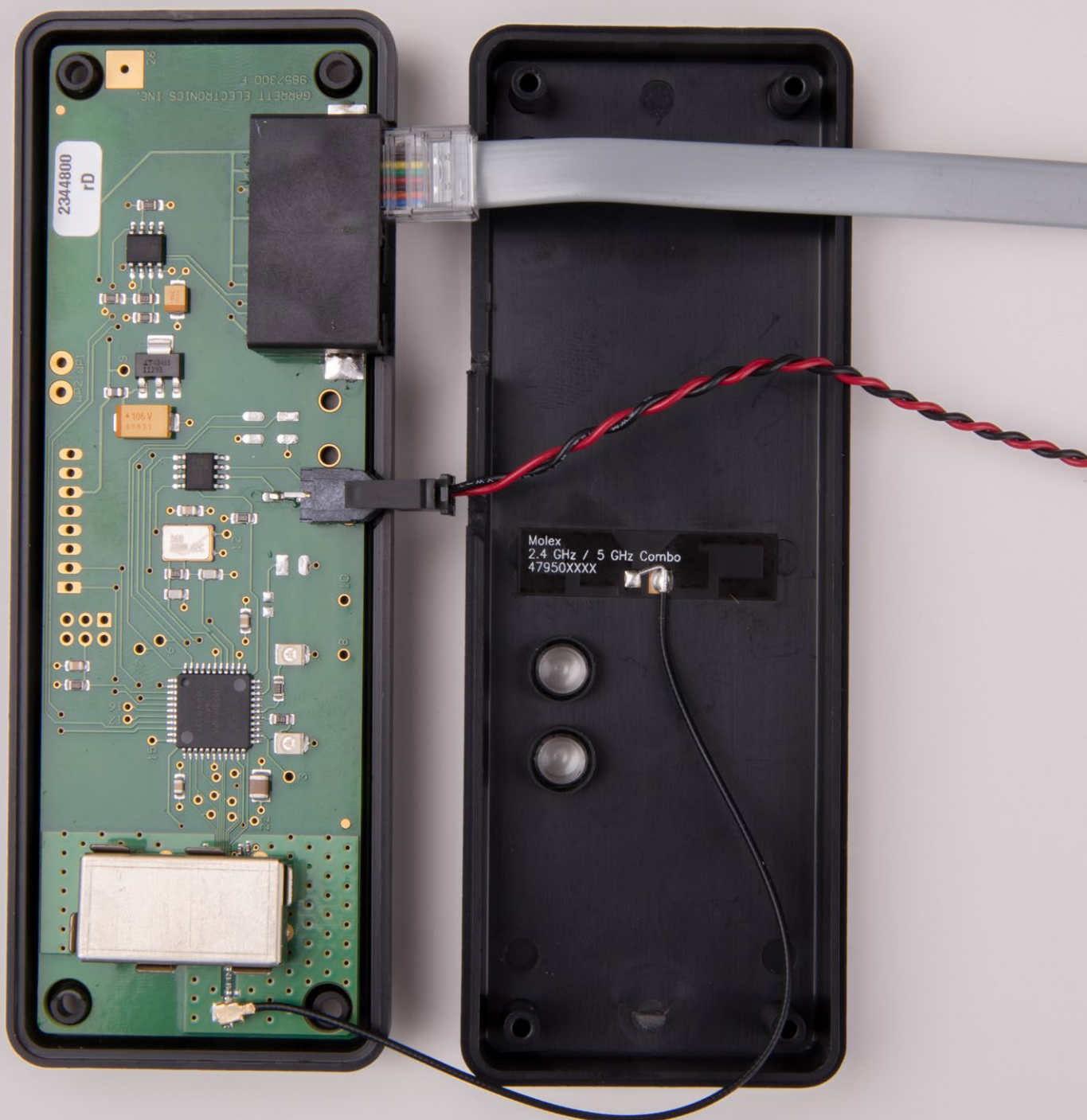
Patch Antenna
