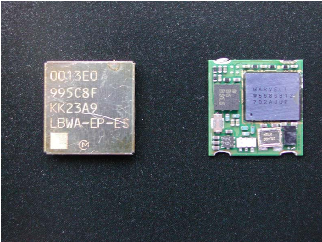
RF part without shield
