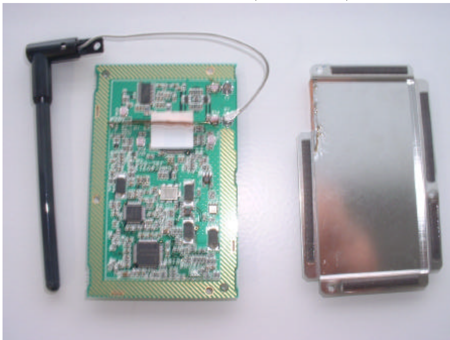
RF Circuit Board (Uncovered)
