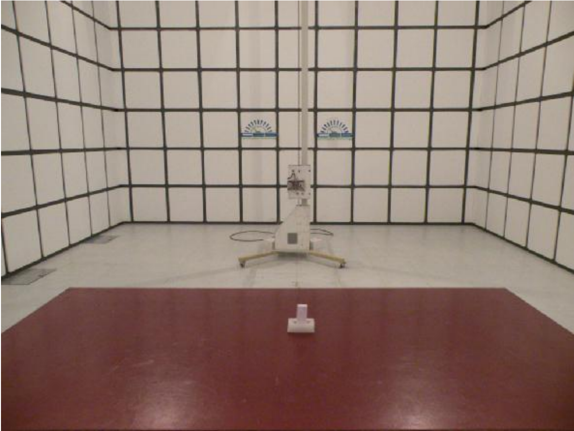
Above 1G test setup photo
