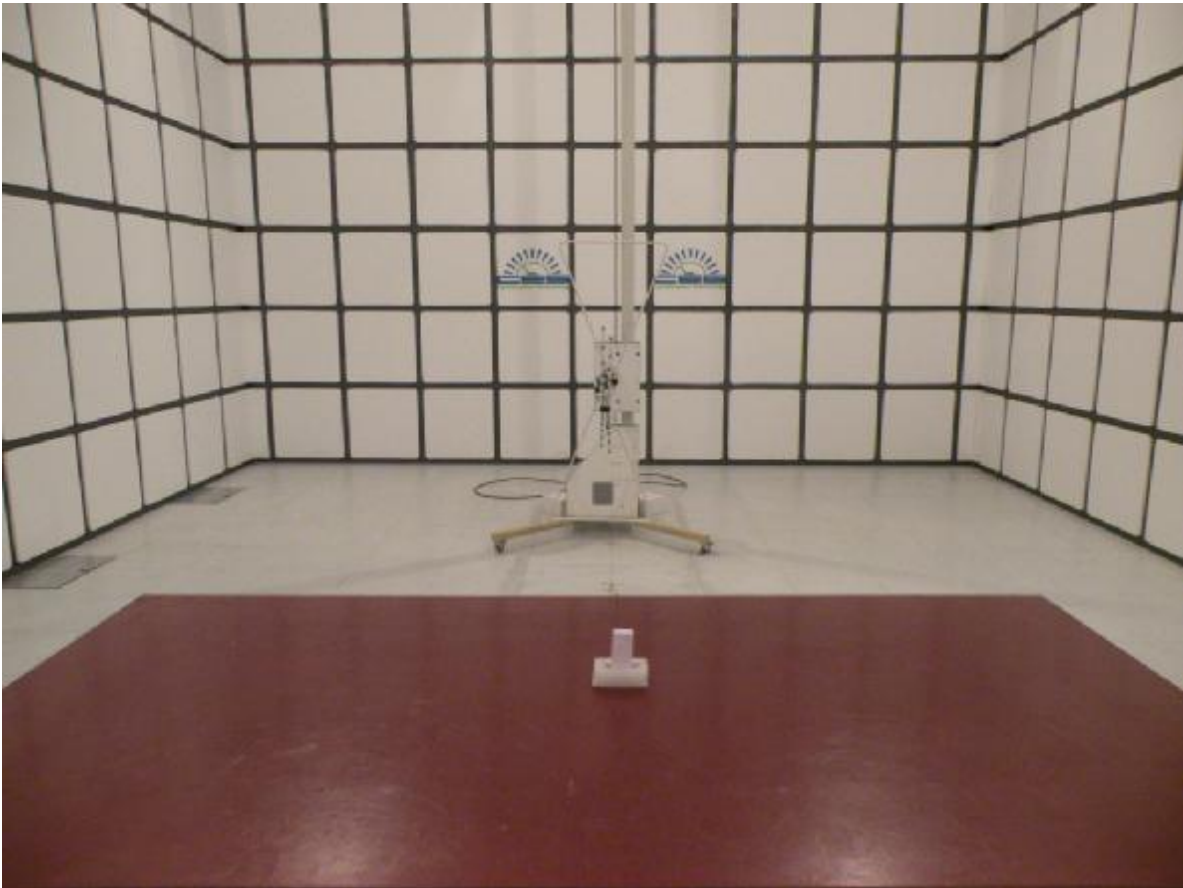
Below 1G test setup photo
