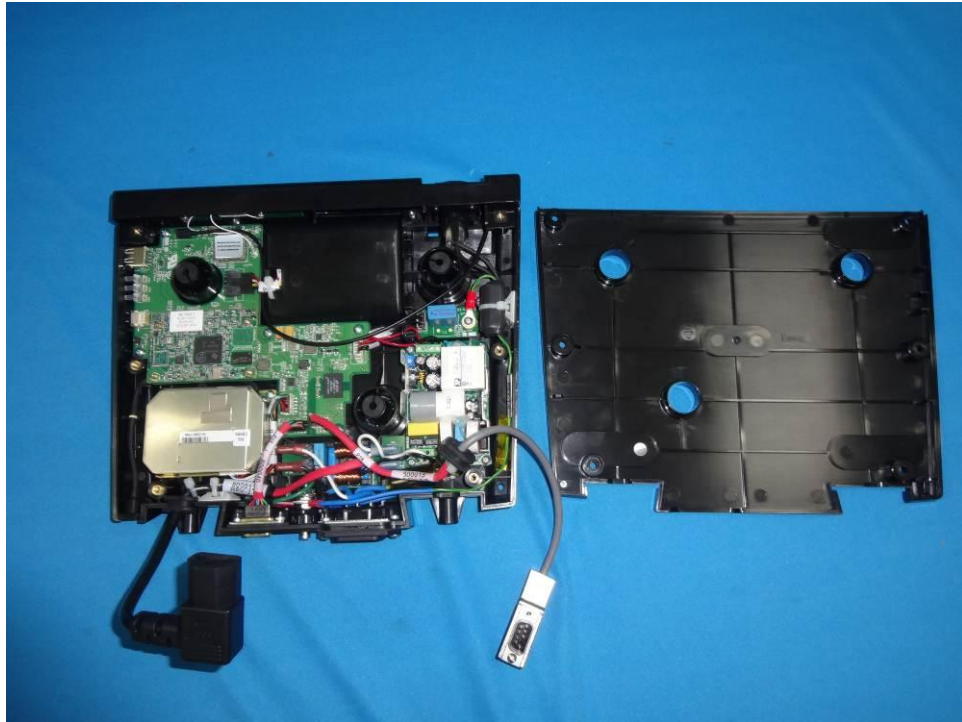
Host Enclosure Opened
