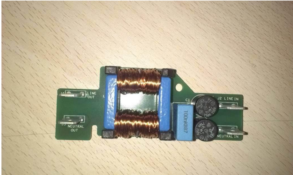
Internal PCB - Host
