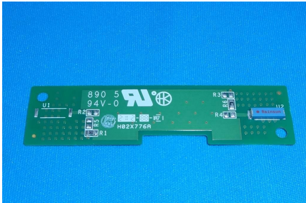
Antenna PCB – Top View
