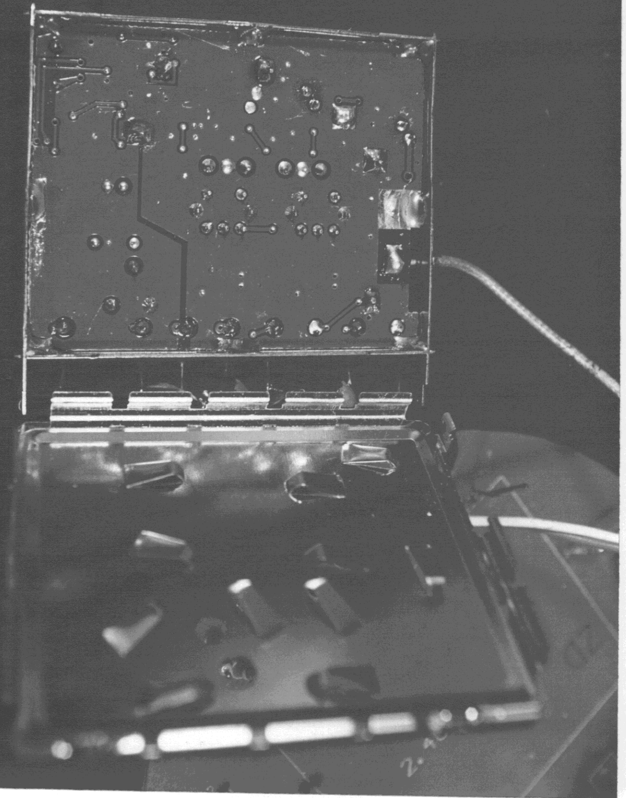
Solder View of RF Module Board
