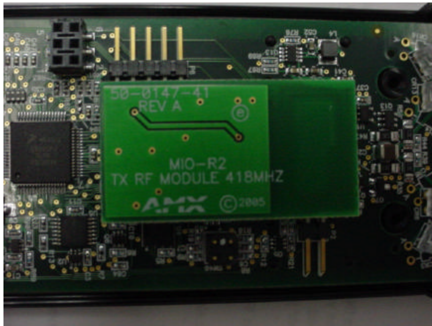
418 Mhz, the MIO-R2 Remote Control/ Module
