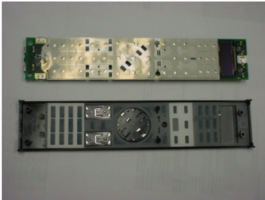
Close up look at the MIO-R2 Remote Control
