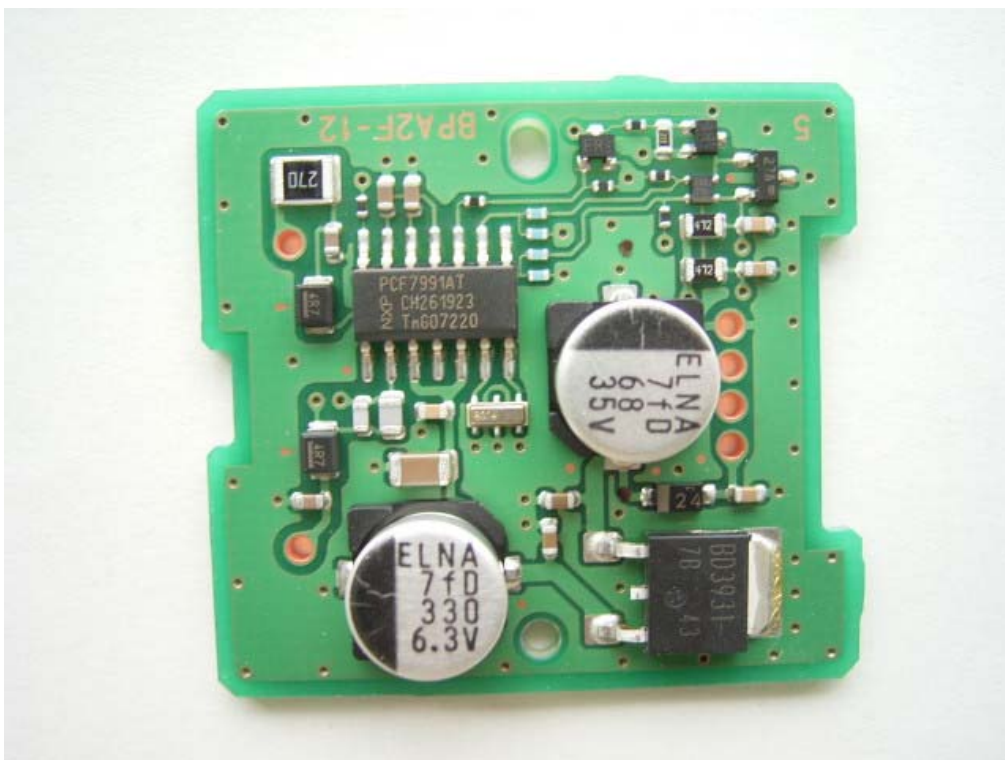
PWB side B
