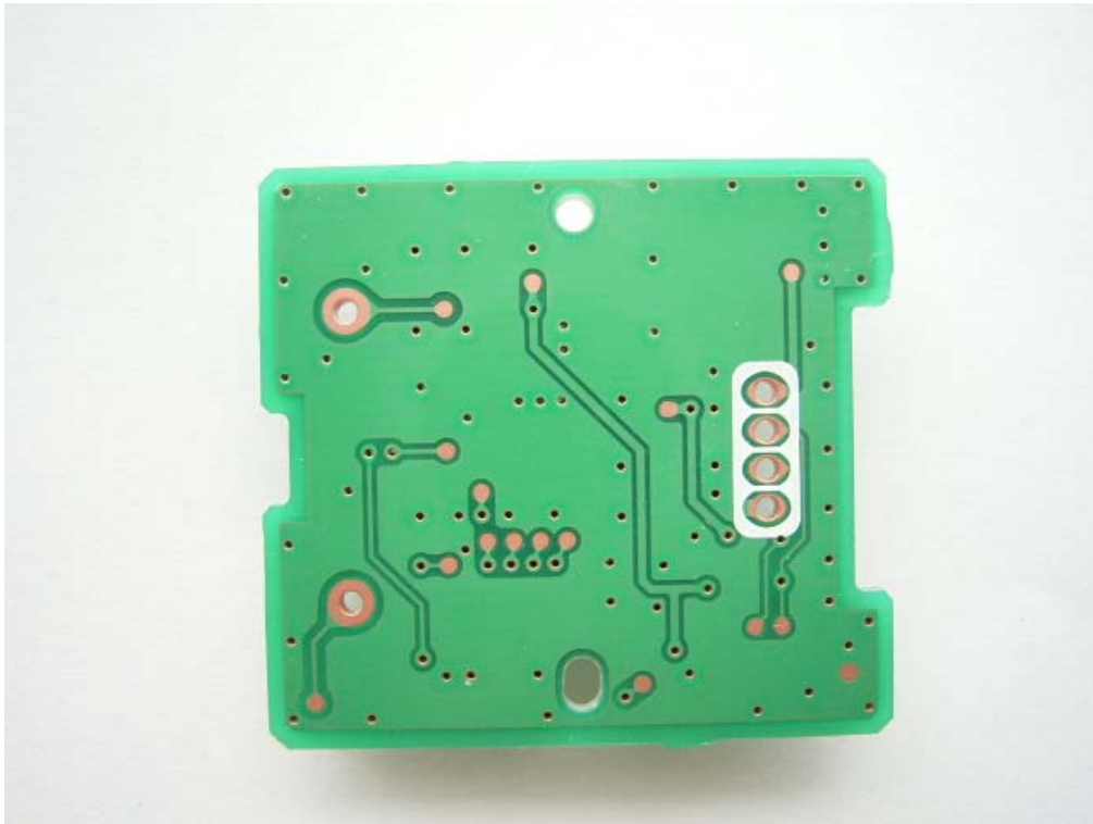
PWB side A
