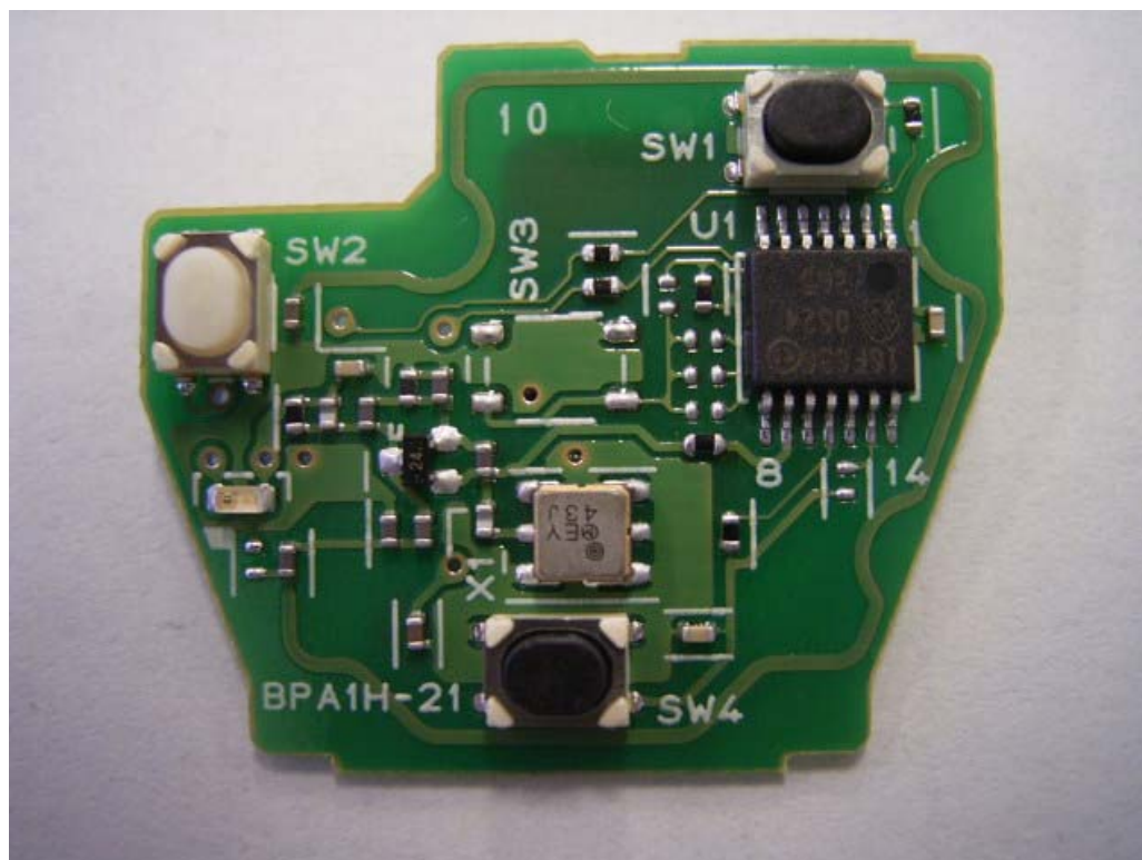
Component Side
