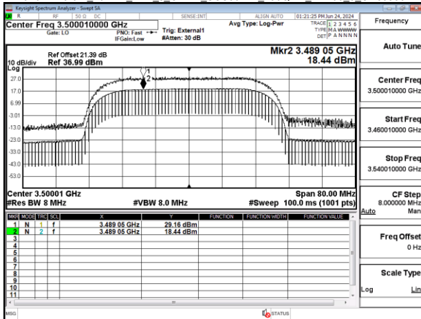
Band77-Part27 40MHz DFT s OFDM_SCS30kHz 256QAM_RB100_0 CH633332
