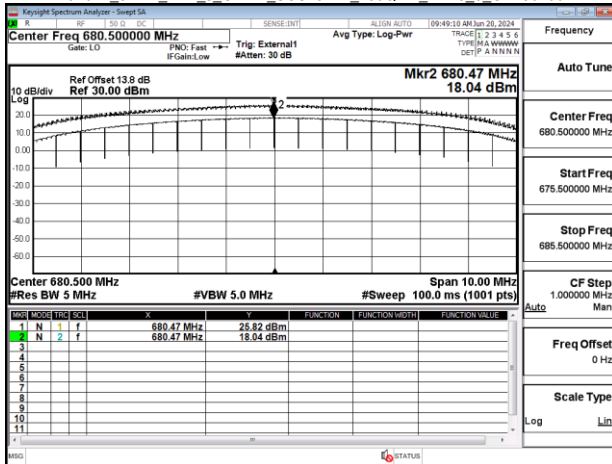
Band71_5MHz_DFT_s_OFDM_SCS15kHz_256QAM_RB25_0_CH136100
