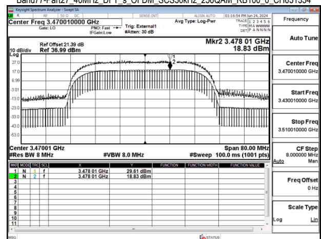
Band77-Part27_40MHz_DFT_s_OFDM_SCS30kHz_256QAM_RB100_0_CH631334
