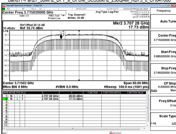
Band77-Part27_30MHz_DFT_s_OFDM_SCS30kHz_256QAM_RB75_0_CH647668
