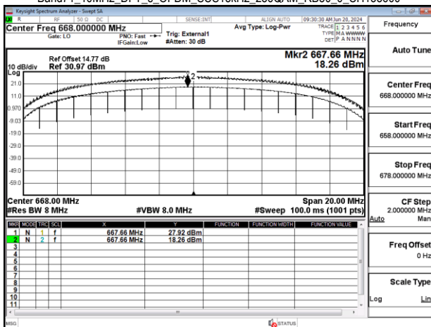
Band71_10MHz_DFT_s_OFDM_SCS15kHz_256QAM_RB50_0_CH133600
